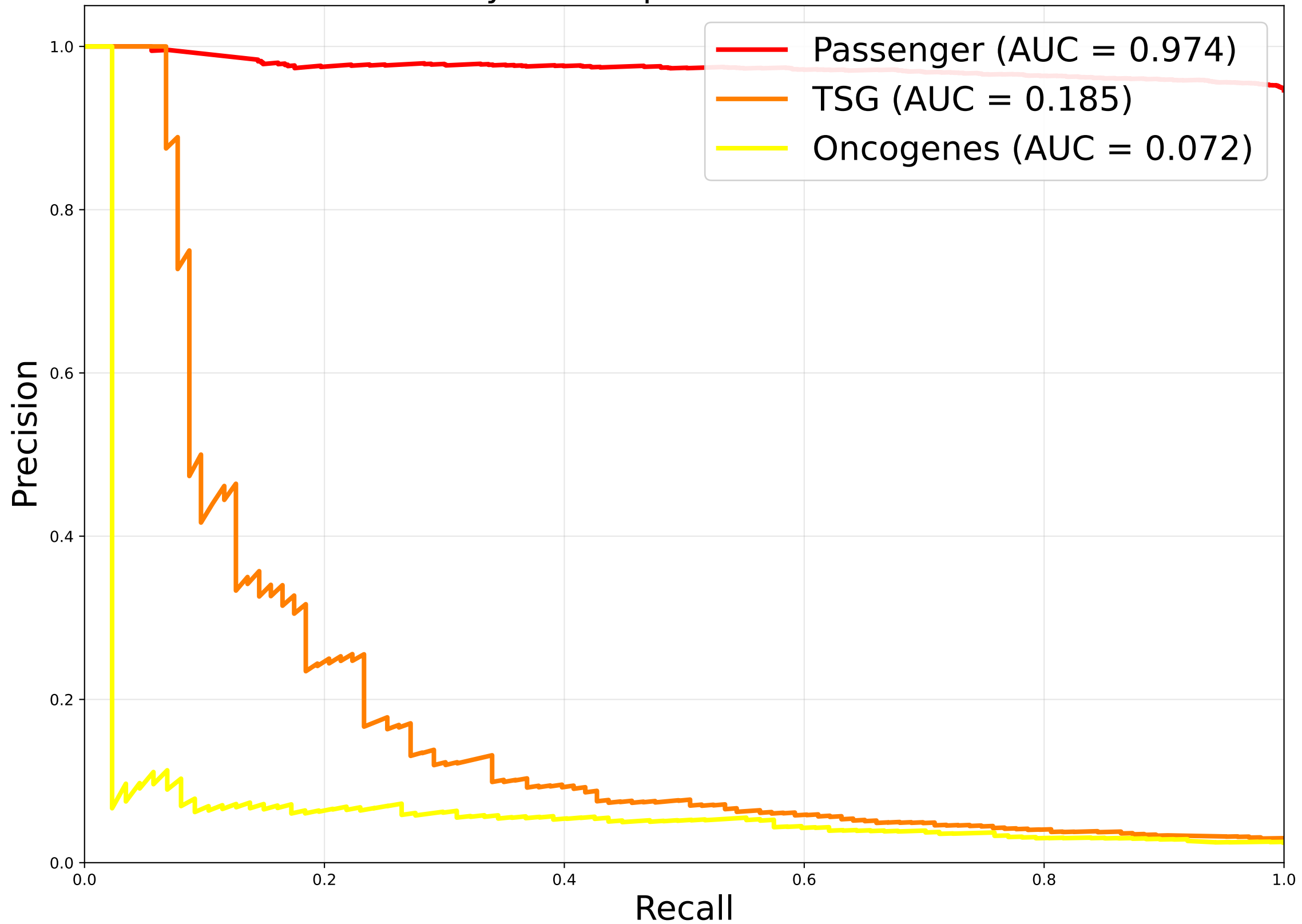
Multi-Layer Perceptron - OvR PR Curves
