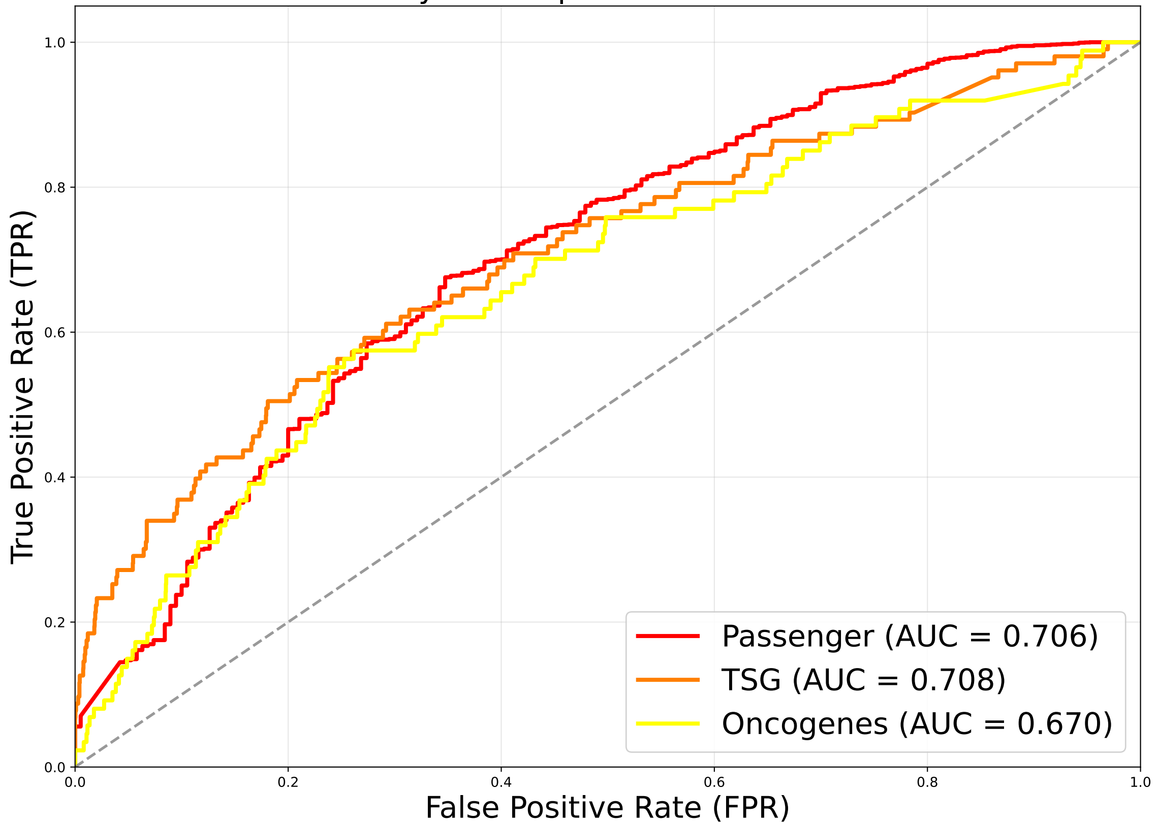
Multi-Layer Perceptron - OvR ROC Curves
