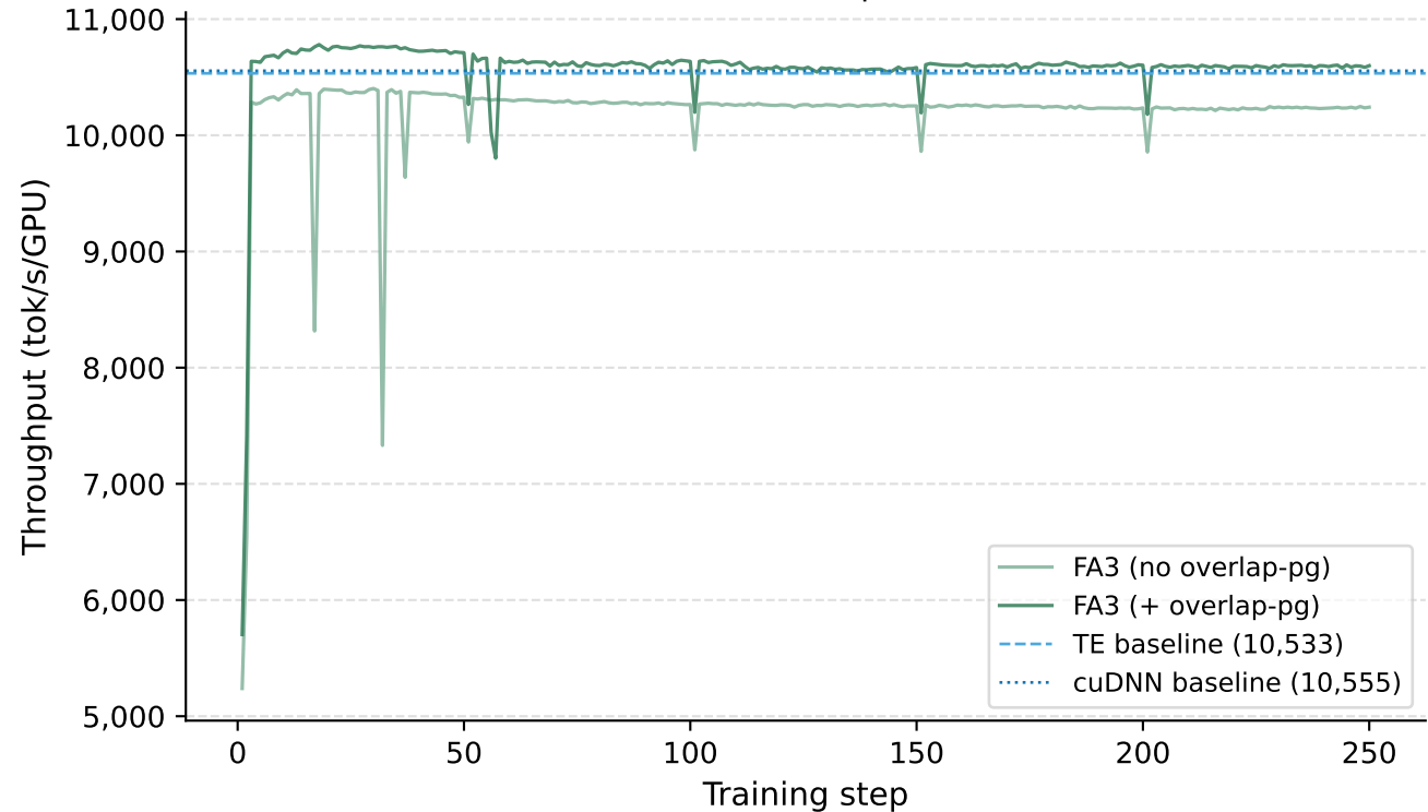
FA3 throughput over training - 4 nodes / 16 GH200 GPUs LLaMA-8B, seq=4096
