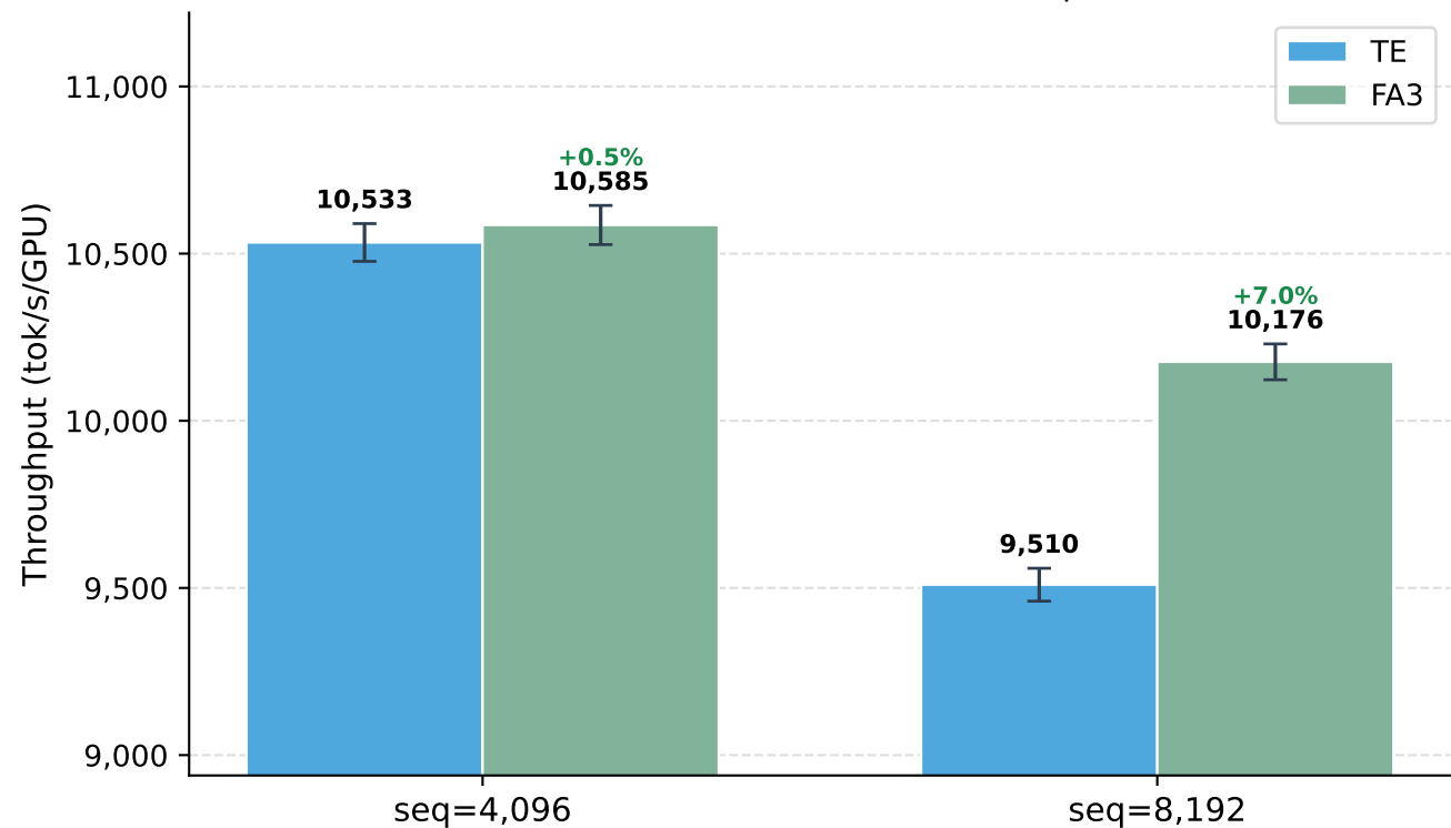
TE vs FA3 throughput scaling with sequence length LLaMA-8B, 4 nodes / 16 GH200 GPUs, steps 200-250
