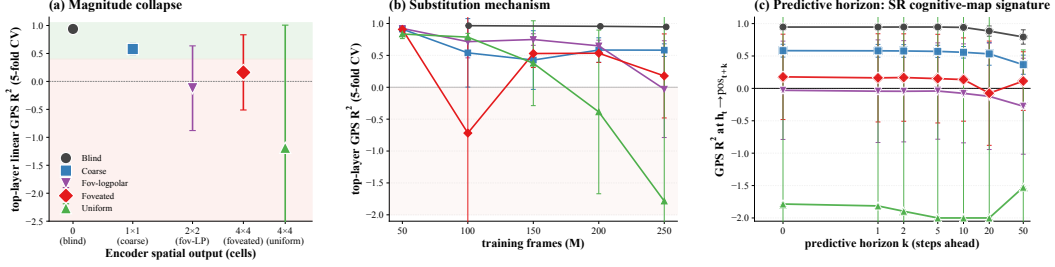
Figure 2: Magnitude axis: linear position decode collapses with encoder bandwidth, develops over training, and only blind retains a long predictive horizon over future positions. (a) Linear GPS R^2 at h_2 falls monotonically with encoder bandwidth (5-fold CV); foveated-logpolar at \sim 2 \times 2 lands in the rich regime. (b) The collapse develops over training only for rich-encoder conditions; bottleneck conditions hold the linear code throughout. (c) Predictive horizon: R^2 of decoding \text{pos}_{t+k} from h_t at lags k \in \{0, \dots, 50\} steps ahead — the canonical Stachenfeld 2017 SR cognitive-map signature. Blind sustains R^2 \gtrsim 0.79 to k=50 ; coarse holds a moderate horizon; rich-encoder conditions show no predictive horizon. Post-retrain hp-consistent agents (Appendix A); panel-level detail in Appendix Figures 30, 31.
