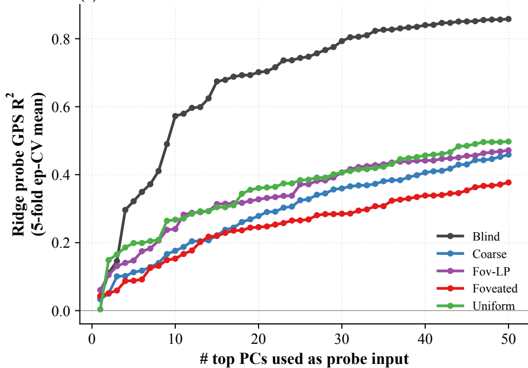
(a) Linear readout vs. # PCs
