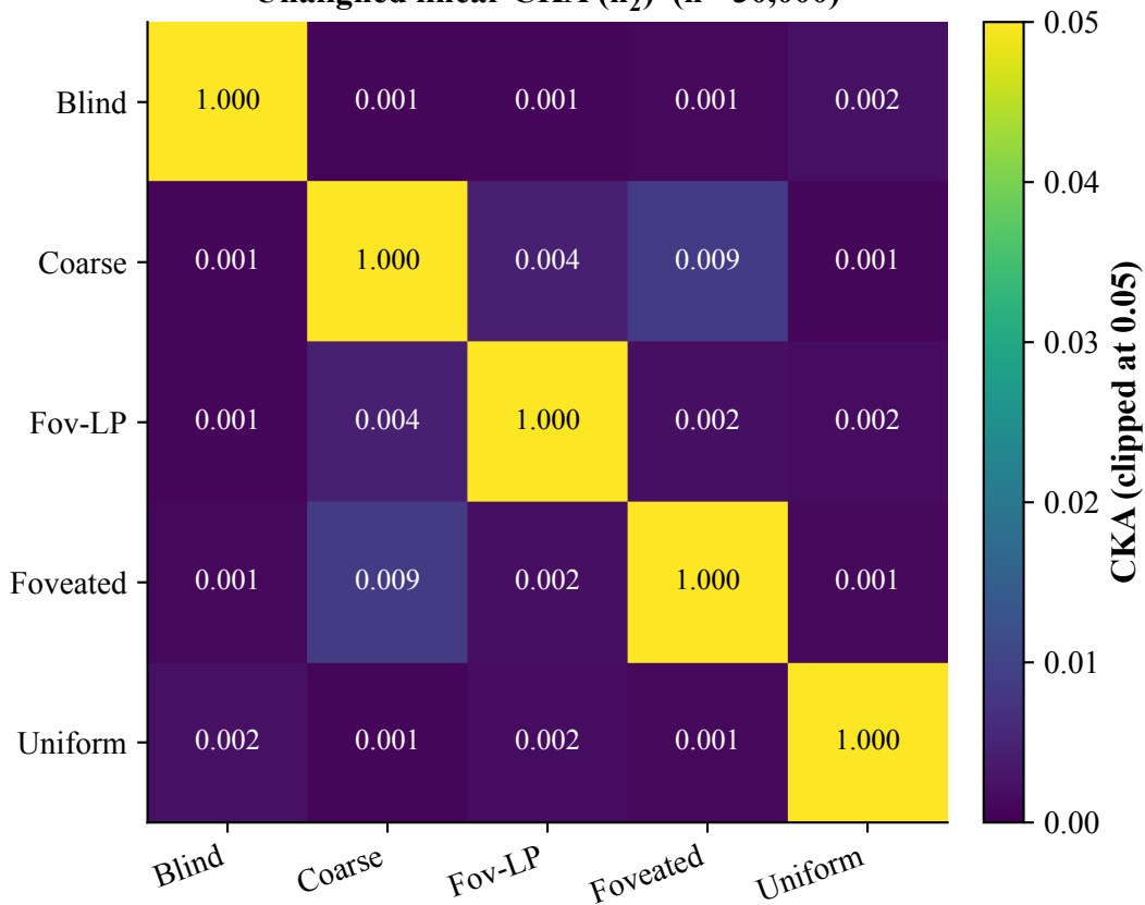
Unaligned linear CKA ( h_2 ) (n=30,000)
