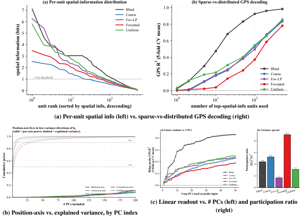
Figure 15: Capacity-allocation geometry within h_2 . (a) Population coding. Per-unit spatial-information distribution per condition (units sorted by spatial information, descending; \log x ): rich-encoder conditions have a few more peaked spatially-tuned units (max \approx 2 bits) than bottleneck conditions, but sparse-vs-distributed GPS decoding (right sub-panel) goes the opposite way — blind reaches R^2 \approx 1.0 with the top- k spatial-info units, while rich-encoder networks fail to decode GPS at any k . Higher per-unit spatial information \neq population position readout: rich-encoder peaked units encode features correlated with position (visual landmarks, trajectory phase) rather than position itself. (b) Position-axis lives in the low-variance tail. Solid: cumulative power of the Ridge-probe singular directions (the linear position-axis) vs. # PCs. Dashed: cumulative explained variance. The manifold’s variance is concentrated in \sim 7 – 9 top PCs (90% by PC 9), but the position-axis distributes its power across 200+ PCs and does not reach 50% within the first 200 PCs. The discriminator across conditions is therefore not where (in a high-variance sense) position lives but the cross-scene stability of the readout direction (Figure 3b). (c) Linear readout vs. # PCs and participation ratio. Ridge-probe GPS R^2 as a function of the number of top PCs of h_2 used as the probe input: blind plateaus quickly with \leq 10 PCs (axis aligned with low-variance dirs); rich-encoder conditions barely climb across 50 PCs (information distributed). The participation ratio (\Sigma \lambda)^2 / \Sigma \lambda^2 is similarly compact across conditions; what differs is how position information is laid out within these dimensions.
