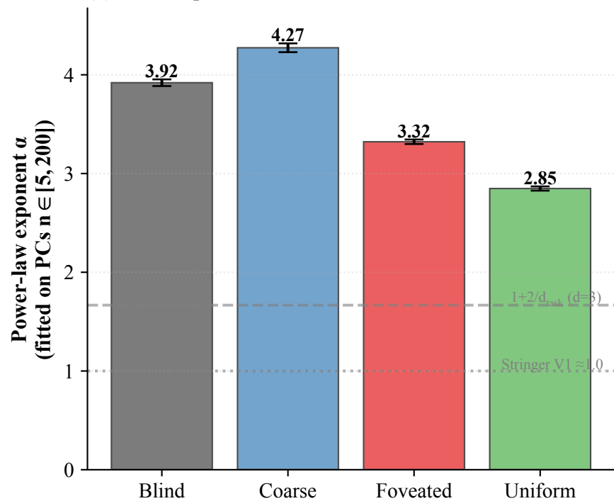
(b) Fitted \alpha per cond
