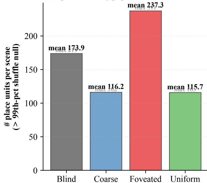
(b) Spatial-coding population size
