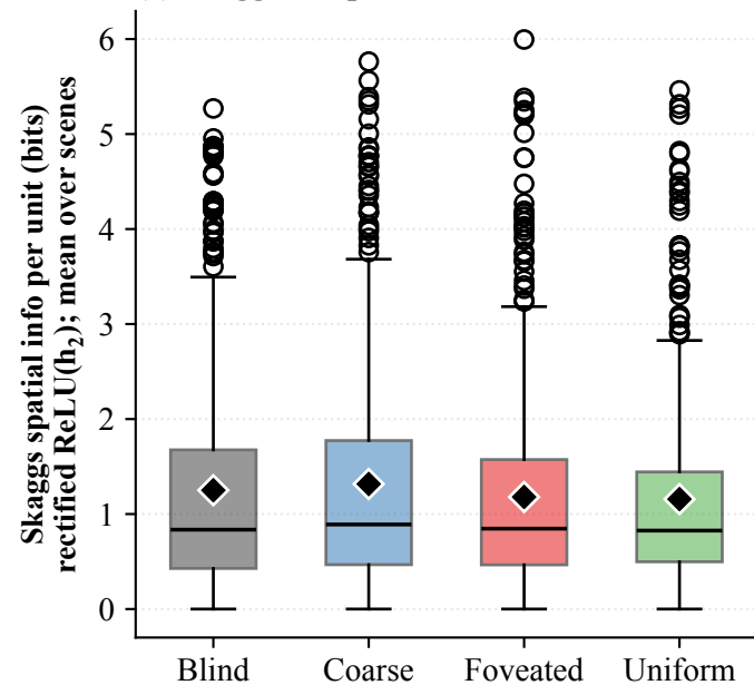
(a) Skaggs bits per LSTM unit
