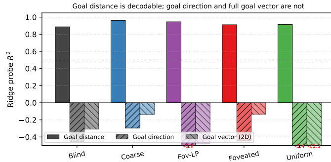
Figure 17: Goal-vector probe R^2 . All five conditions. Goal distance (DtG) decodes strongly everywhere ( R^2 \in [0.89, 0.96] , 5-fold CV); goal direction and the full ego-frame goal vector are at chance or negative for every condition. PointGoal provides the goal vector as a per-step input, so the policy has no incentive to re-encode it.
