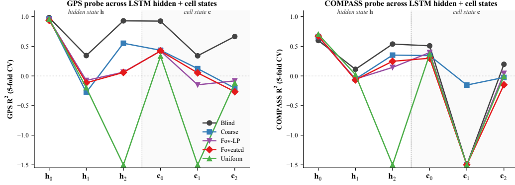
Figure 10: Where GPS lives along the LSTM stack: per-layer linear probe R^2 . 5-fold CV linear probe at each hidden state h_\ell and cell state c_\ell , \ell \in \{0, 1, 2\} , all five conditions (Blind, Coarse, Fov-LP, Foveated, Uniform). Left: GPS. Right: compass. At h_0 all conditions decode GPS at R^2 \sim 0.95 — the GPS sensor embedding enters the LSTM concat at Layer 0 regardless of vision condition. h_1 dips for every condition including blind ( R^2 = +0.22 ); information passes through the middle layer with reduced linear decodability for everyone, then partly recovers at h_2 for the bottleneck conditions. Cell states c_\ell do not carry the GPS code as cleanly as h_\ell : c_1 is at chance/negative for every condition; c_2 is positive only for blind ( R^2 = +0.57 ). The headline “top-layer linearly-decodable GPS” result in §3.1 is therefore specifically about h_2 (the policy readout), not the cell-state pathway.
