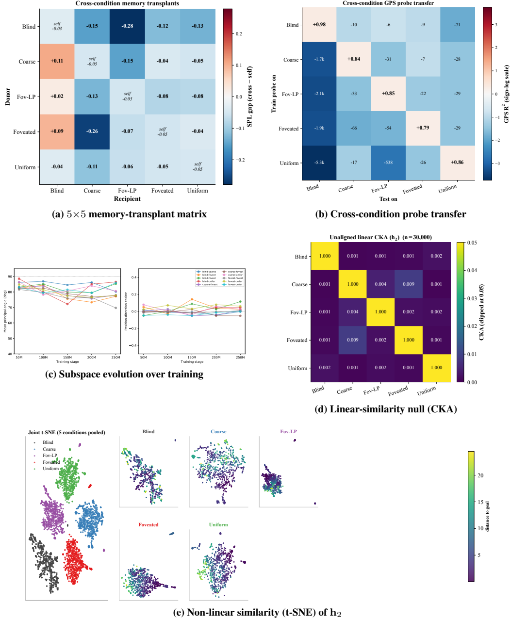
Figure 14: Format divergence: five convergent metrics. (a) Full 5 \times 5 memory-transplant matrix at midpoint t=30 (the per-recipient mean enters main Figure 3b as the transplant-cost axis); the matrix shows the same direction-asymmetry condensed there. (b) Cross-condition probe transfer matrix (train on row, test on column): off-diagonal R^2 is catastrophically negative ( -3.5 \times 10^2 to -3.5 \times 10^4 unclipped; clipped to [-1, 1] here) — position-axes are jointly incompatible at the readout level even when the same scenes are visited and the same task is solved. (c) Principal angles between conditions’ position-direction subspaces over training: already near-orthogonal at the earliest probed checkpoint ( \sim 50 M frames) and stay so throughout, so the structural separation is laid down well before convergence. (d) Unaligned linear CKA [Kornblith et al., 2019] between top-layer LSTM hidden states ( n=95,640 steps/cond): every off-diagonal < 10^{-4} ; within-condition split-half CKA \approx 1 . CKA is the least informative of the five measures because it cannot read the asymmetric structure that transplant + probe-transfer show. (e) t-SNE of top-layer hidden states (perplexity 30, 5,000 samples; left: joint embedding, 1-NN purity 1.000 vs. chance 0.20; right: per-condition embedding coloured by distance-to-goal). Blind shows the clearest DtG gradient, consistent with its more directly readable position code.
