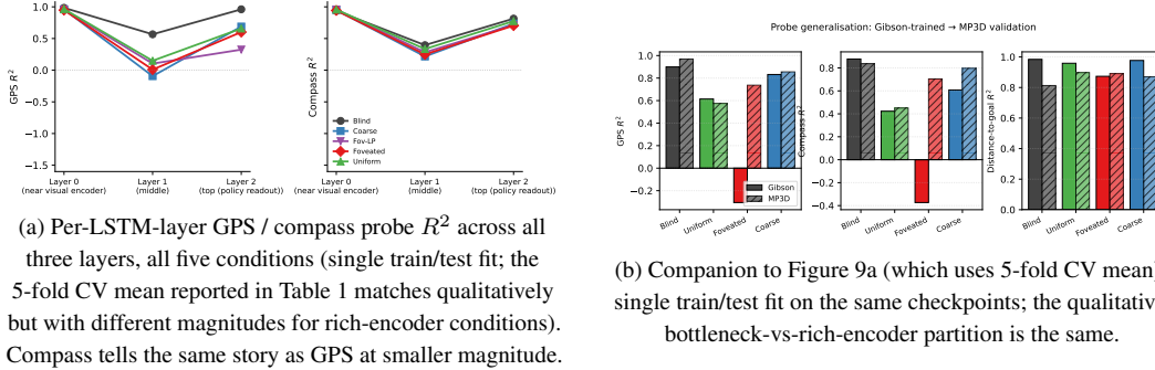
Figure 11: Single-fit per-layer and MP3D companion checks. Companion to the headline 5-fold CV results: a single train/test split reproduces the bottleneck-vs-rich-encoder partition reported in Table 1, ruling out CV-fold-induced artefacts. The MP3D panel re-evaluates the same checkpoints on a held-out scene distribution; the partition still holds.
