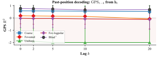
Figure 3. GPS R^2 for past-position probes \text{GPS}_{t-k} from current \mathbf{h}_t . Uniform’s mean R^2 falls below the visible range from k=5 onward (true values -2.28, -3.01, -6.53 at k=5, 10, 20 ); shown clipped at -2.0 . Blind point: preliminary 100-ep partial NPZ.
