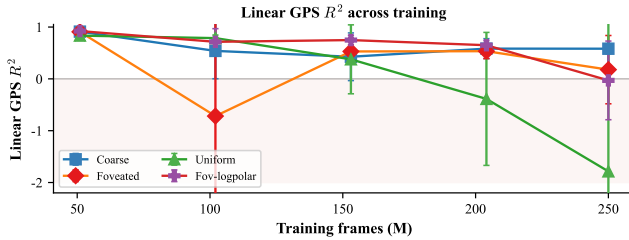
Figure 2. Linear GPS R^2 at 5 training checkpoints per sighted condition (blind omitted: only the 340M endpoint checkpoint is available, no intermediate blind checkpoints exist for a trajectory). Negative- R^2 outliers clipped to -2.0 .
