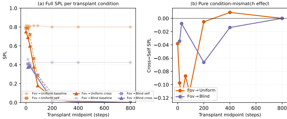
Figure 9: Memory-transplant midpoint sweep on two representative donor \rightarrow recipient pairs (foveated \rightarrow uniform, foveated \rightarrow blind) across midpoints \{0, 15, 30, 60, 90, 200, 400, 800\} time-steps ( n=100\text{--}150 episodes/cell). The full 5\times 5 matrix in Figure 5 (right) is at midpoint t=30 . (a): full SPL per condition — baseline / self / cross. The t=0 self/cross collapse to a protocol-noise floor (so the diagonal in Figure 5 is correctly read as rollout-divergence noise, not condition mismatch); SPL decays for all conditions at t \geq 200 because by then most successful episodes have already terminated, leaving only long atypical episodes. (b): cross-minus-self isolates condition-mismatch alone. The gap peaks in the t \in [30, 90] window — where the agent has integrated history but is not yet committed to a trajectory — and decays toward 0 at t \geq 400 . The asymmetry pattern reported at t=30 in Figure 5 is therefore neither a t=30 -specific artefact nor a late-midpoint inflation.
