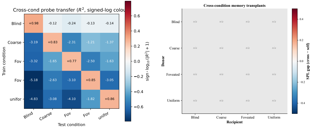
Figure 8: Subspace divergence ( H_2 ), two views. Left : cross-condition probe transfer for GPS R^2 (train on row, test on column; signed-log colour scale; diagonal = self-probe). Right : 4 \times 4 cross-condition memory-transplant matrix at midpoint t=30 ; off-diagonal = cross-transplant SPL – recipient’s self-transplant SPL. Single seed; midpoint-sweep companion in Appendix E.
