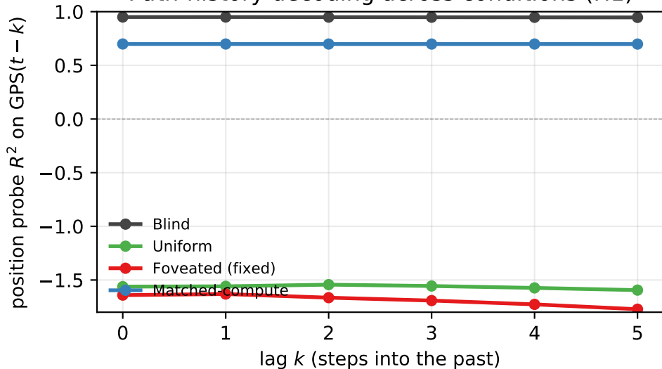
Path-history decoding across conditions (H1)
