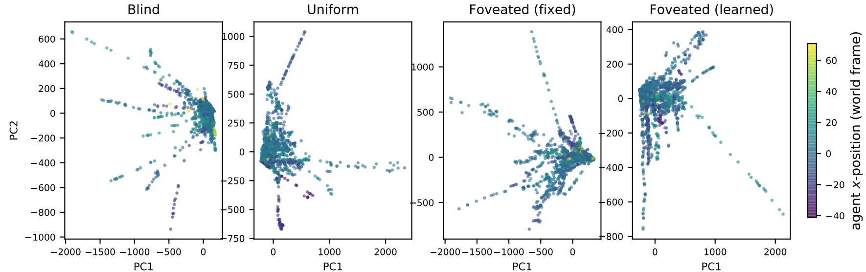
Per-condition PCA of top-layer LSTM hidden state, coloured by agent position
