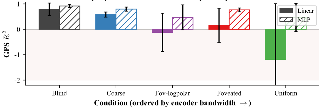
Top-layer GPS R^2 : linear vs MLP probe by condition
