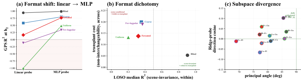
Figure 3: Three views of the format axis. (a) Format shift : slope chart from Linear to MLP probe per condition; steep slope = large gap between linear and non-linear readability. Bottleneck conditions sit on near-horizontal slopes; rich-encoder conditions on near-vertical ones — a format shift, not an information loss. (b) Format dichotomy : LOSO median R^2 (within-condition scene-invariance) vs. mean cross-condition transplant cost (across-condition non-interchangeability). Bottleneck (blind) sits in the scene-invariant + transplant-robust quadrant; rich-encoder conditions cluster in the scene-conditional + transplant-brittle quadrant. (c) Subspace divergence : all 10 condition pairs plotted by principal angle (between top- K PCA subspaces) and Ridge-probe direction-cosine. All cluster near (90^\circ, 0) — the “fully orthogonal” target — geometrically corroborating the behavioural transplant test in (b).
