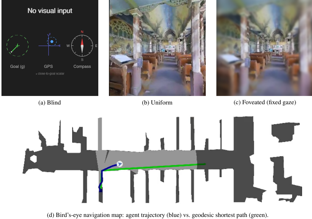
Figure 1: The five visual conditions differ only in what reaches the agent’s encoder. (a) Blind : no visual input; only the non-visual sensor stack (goal-in-start-frame, GPS, compass, close-to-goal scalar) — the Wijmans [Wijmans et al., 2023] configuration. (b) Uniform : 256 \times 256 full-resolution RGB. (c) Foveated (fixed gaze) : eccentricity-dependent Gaussian blur centred on the image middle ( \sigma_{\max} = 8 , quadratic falloff). The two additional conditions not shown are matched-compute (a down-sampled uniform view with the same total pixel budget as foveated) and foveated (learned gaze) , which adds a learned (x, y) gaze offset to (c). (d) All conditions solve PointGoal navigation in the same Habitat Matterport3D / Gibson scenes; the top-down view is shown for reference only and is not available to the agent.
