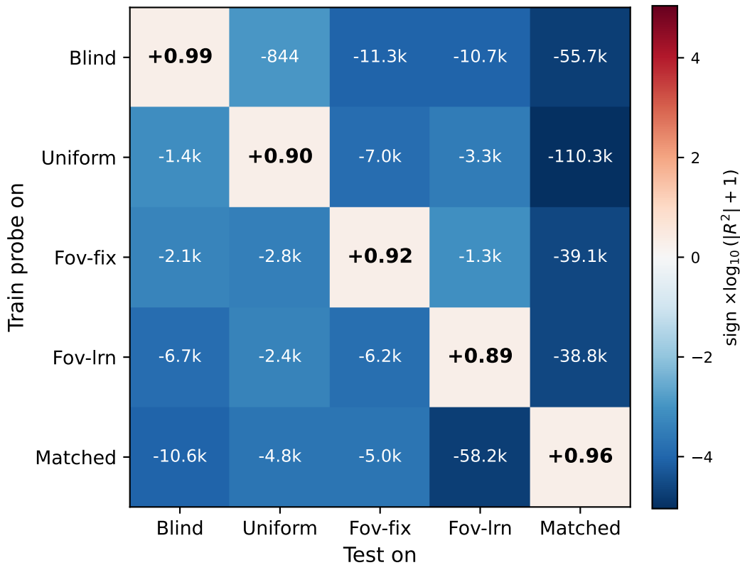
Cross-condition probe transfer (GPS R^2 ) diagonal = self-probe, off-diagonal = off-manifold
