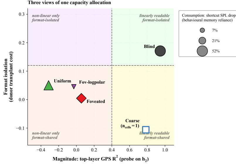
Figure 6: Three views of one capacity allocation, one point per condition. X axis: magnitude (top-layer GPS R^2 on h_2 , §??). Y axis: format isolation (donor transplant cost, §??; higher Y = donor memory is more disruptive to other conditions’ policies). Marker size: consumption (shortcut SPL drop, §??; larger = more policy reliance on persistent memory). Coarse’s Y has only n_{\text{cells}}=1 (single donor cell available, hollow marker).
