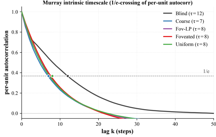
Figure 18: Murray-style intrinsic timescale per condition. Per-unit autocorrelation curves averaged over 256 random units \times 80 random episodes per condition; coloured dot marks the lag at which each curve crosses 1/e (the intrinsic timescale \tau ). Blind \tau \approx 12 ; every sighted condition \tau \approx 7 –8.
