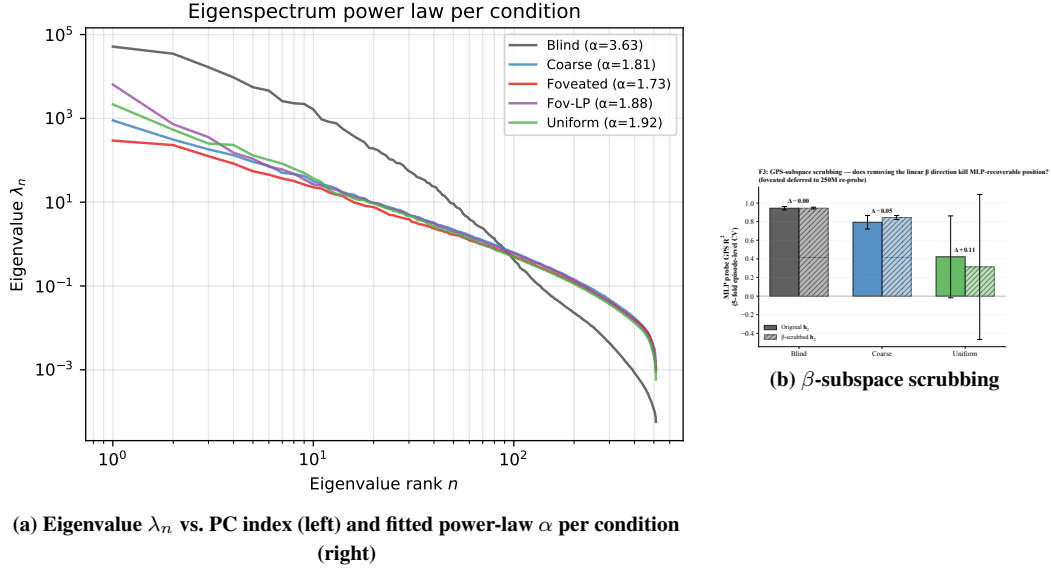
Figure 16: Eigenspectrum and causal redundancy of the position code. (a) Eigenvalue \lambda_n vs. PC index n for \mathbf{h}_2 , log-log (reference exponents \alpha = 1 , Stringer V1; \alpha = 1 + 2/3 , theoretical critical exponent for d_{\text{task}}=3 ); fitted exponent \alpha per condition (linear fit on \log-\lambda_n vs. \log-n , PCs 5–200). Blind sits well above the critical exponent ( \alpha \approx 3.85 , top-10 PCs capture 95% variance), in a few-dim concentrated regime; the four sighted conditions cluster around \alpha \approx 1.7 – 1.9 , near the smoothness/efficiency border, distributing hidden-state variance across more directions. The split is the geometric reading of the capacity-allocation principle: blind’s heavy reliance on the integrated GPS code crystallises into a low-dimensional eigenspectrum; sighted conditions distribute variance across more directions to support encoder-route information. (b) \beta -subspace scrubbing. Ridge \beta identifies a 2-d direction in \mathbf{h}_2 that linearly predicts (x, y) ; scrubbed \mathbf{h}_2 = (I - \beta^+ \beta) \mathbf{h}_2 removes this 2-d subspace. The MLP probe is essentially unaffected: position information is redundantly distributed across many \mathbf{h}_2 dimensions, not concentrated in the 2-d \beta subspace — the population-coding-redundancy property of biological place-cell systems (?). (Cache for (b): Blind / Coarse / Uniform.)
