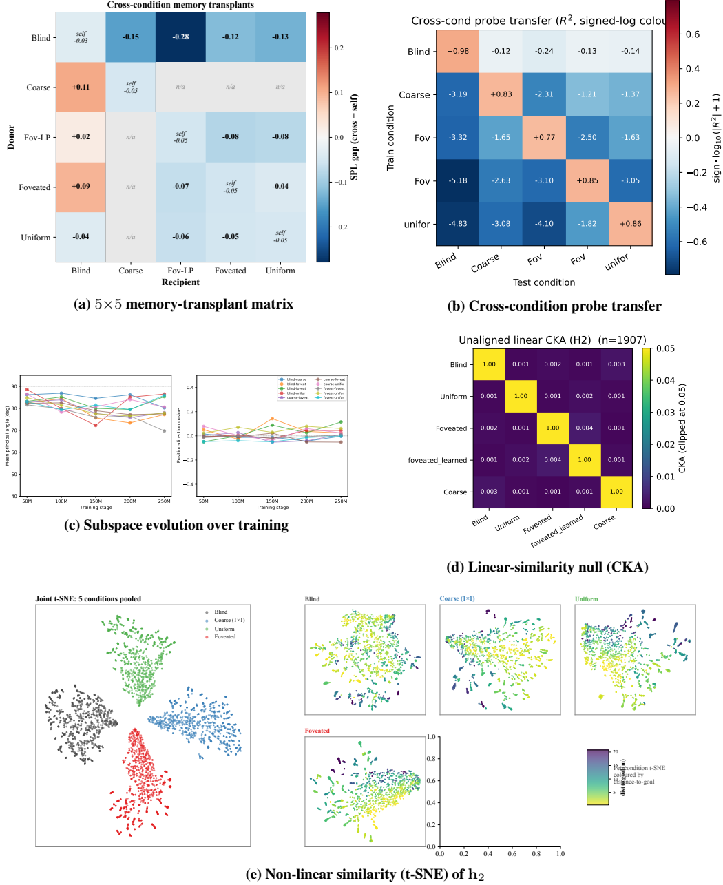
Figure 14: Format divergence: five convergent metrics. (a) Full 5 \times 5 memory-transplant matrix at midpoint t=30 (the per-recipient mean enters main Figure ??b as the transplant-cost axis); the matrix shows the same direction-asymmetry condensed there. (b) Cross-condition probe transfer matrix (train on row, test on column): off-diagonal R^2 is catastrophically negative ( -3.5 \times 10^2 to -3.5 \times 10^4 unclipped; clipped to [-1, 1] here) — position-axes are jointly incompatible at the readout level even when the same scenes are visited and the same task is solved. (c) Principal angles between conditions’ position-direction subspaces over training: already near-orthogonal at the earliest probed checkpoint ( \sim 50M frames) and stay so throughout, so the structural separation is laid down well before convergence. (d) Unaligned linear CKA (?) between top-layer LSTM hidden states ( n=95,640 steps/cond): every off-diagonal < 10^{-4} ; within-condition split-half CKA \approx 1 . CKA is the least informative of the five measures because it cannot read the asymmetric structure that transplant + probe-transfer show. (e) t-SNE of top-layer hidden states (perplexity 30, 5,000 samples; left: joint embedding, 1-NN purity 1.000 vs. chance 0.20; right: per-condition embedding coloured by distance-to-goal). Blind shows the clearest DtG gradient, consistent with its more directly readable position code. (Cache: panels d, e use 4 conditions; fov-LP omitted.)
