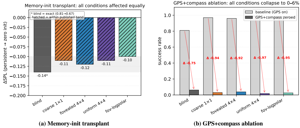
Figure 20: Boundary-check causal interventions. (a) Memory-init transplant: re-initialising memory from the previous episode’s end-state instead of zero drops SPL by a comparable amount across all five conditions. The cross-condition uniformity is the finding — every agent’s policy expects a zero memory state at t=0 , so memory acts as an activity-slot store bound to the trajectory dynamics. (b) GPS+compass ablation: zeroing GPS and compass from step 0 collapses success to near-zero across all conditions. Drops cluster tightly across sighted; blind drops less because its baseline is already lower. The position sensor is the upstream causal source whose integration the memory encodes.
