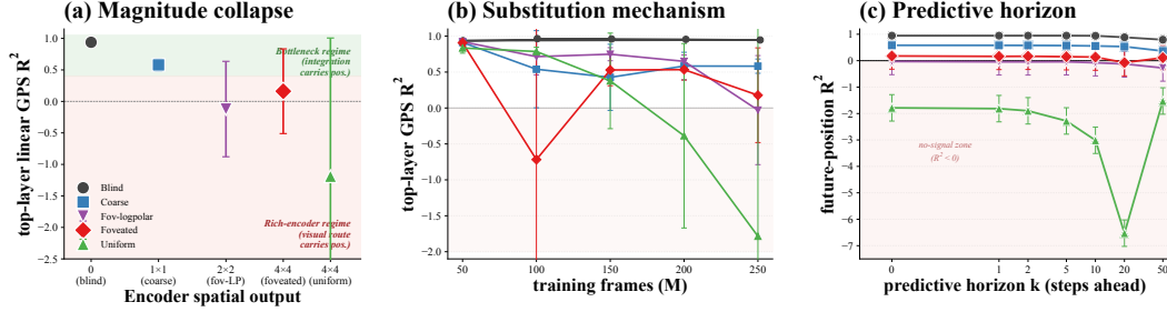
Figure 2: Three views of magnitude. (a) Cross-condition : top-layer linear GPS R^2 falls with encoder bandwidth. (b) Across training : rich-encoder conditions start high then lose readability; bottleneck conditions hold it throughout. (c) Predictive horizon : only bottleneck conditions linearly decode \text{post}_{t+k} at long k . Shaded band: R^2 < 0 , the linear probe is worse than predict-mean baseline — the “no-signal zone”. Uniform’s curve dives deep into this zone (its hidden state is scene-conditional, so 5-fold CV trains on some scenes’ position-directions and tests on incompatible ones, producing systematically negative R^2 ); the dive is noise, not a meaningful trend.
