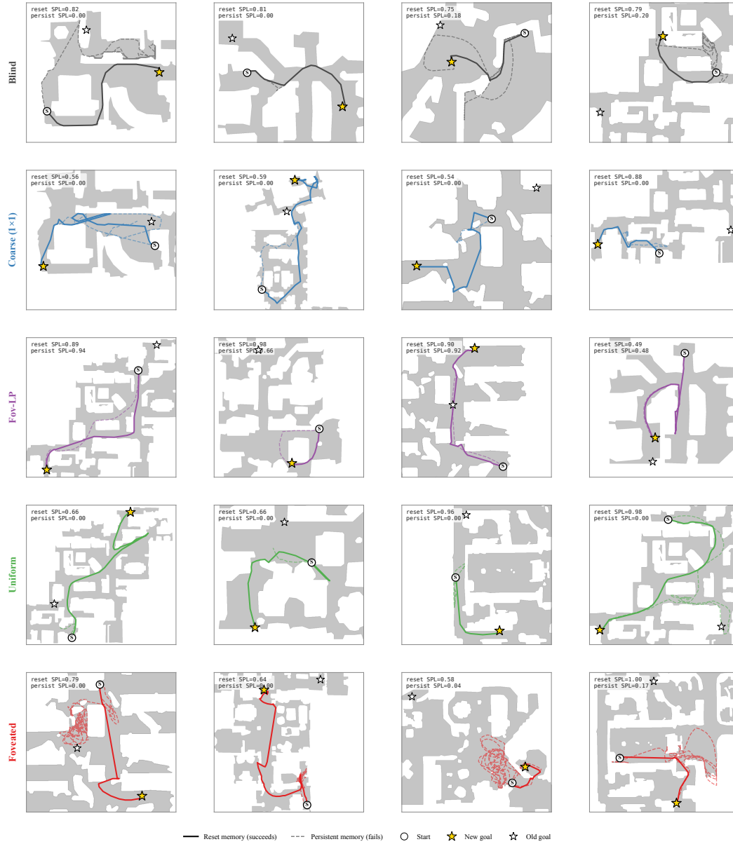
Figure 21: Persistent-memory failure-mode catalog: 4 cases per condition spanning the per-condition margin distribution. Reset trajectory (solid, condition colour) reaches the new goal; persistent trajectory (dashed bold) shows where the persistent-memory agent ends up. Bottleneck conditions (Blind, Coarse) cluster at “tries-new”; Fov-LP also tries-new in all four selected cases (its persistent agent rarely fails to reach the new goal, the “robust to memory carryover” pattern); Uniform clusters at “locks-onto-old”; Foveated is mixed.
