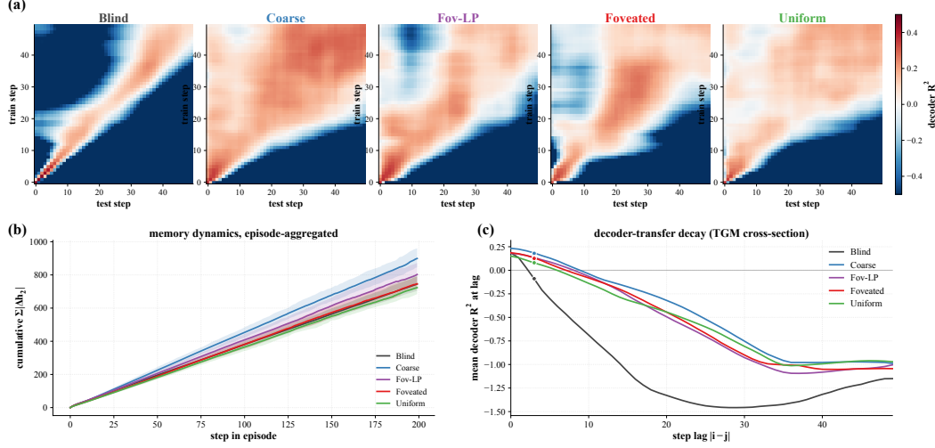
Figure 4: Temporal format: blind rotates the readout axis step by step; sighted hold it stationary, with stiffness graded by encoder bandwidth. (a) Step-by-step decoder generalisation (?): each 50 \times 50 heatmap is decoder R^2 trained at row step, tested at column step. Diagonal-only \Rightarrow rotating basis (blind); square block \Rightarrow stationary readout (coarse); intermediates \Rightarrow fov-LP, foveated, uniform. (b) Cumulative memory displacement \Sigma|\Delta h_2| vs step-in-episode, mean and 25–75 percentile band aggregated over all evaluation episodes per condition: total memory work per step. (c) Mean decoder R^2 vs step lag |i-j| , each panel-(a) TGM collapsed to a curve: format stationarity. Panel (c) ranks coarse +0.18 > fov-LP/foveated +0.13 > uniform +0.08 , the inverse of encoder bandwidth (less bandwidth, more stationary). Murray \tau and persistent-homology corroborations in App ??.
