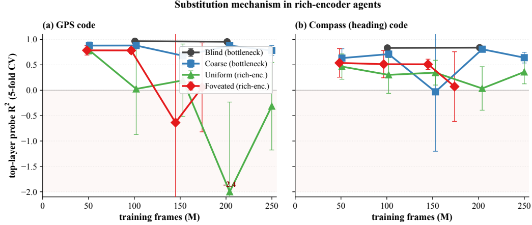
Figure 12: Cross-training substitution dynamics: GPS and compass (companion to main Figure ??b). Probe R^2 across training checkpoints, truncated at 250M frames. (a) Top-layer GPS R^2 (the source panel for Figure ??b). (b) Top-layer compass R^2 tells the same story at smaller magnitude — substitution applies to spatial codes broadly, not just position.
