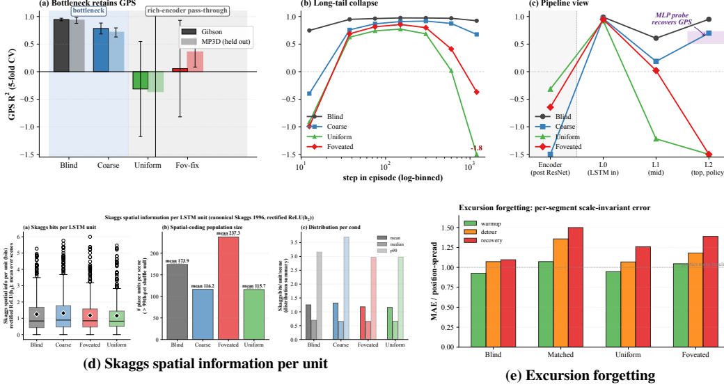
Figure 9: Magnitude: corroborating diagnostics. (a) Top-layer GPS R^2 on Gibson and held-out MP3D (5-fold CV, deterministic rollouts, 300 ep/cond; lighter bars = MP3D). (b) GPS R^2 binned by step-in-episode (7 log-spaced bins): rich-encoder readability holds in the mid-episode window then collapses in the long tail. (c) Pipeline view, single-fit: GPS R^2 along Encoder \rightarrow L0 (LSTM input) \rightarrow L1 \rightarrow L2; readability is comparable at the LSTM input and only diverges at L2 (shaded band at L2: 2-layer MLP probe recovery range). (d) Per-unit Skaggs spatial information (?) is condition-flat; the per-unit regression analysis in §?? (trajectory-phase vs. raw-position R^2 ) is the more diagnostic reading. (e) Mid-episode excursion forgetting (25-step random-action perturbation, per-segment scale-invariant MAE): blind fragments most, consistent with the strongest reliance on the integrated action stream.
