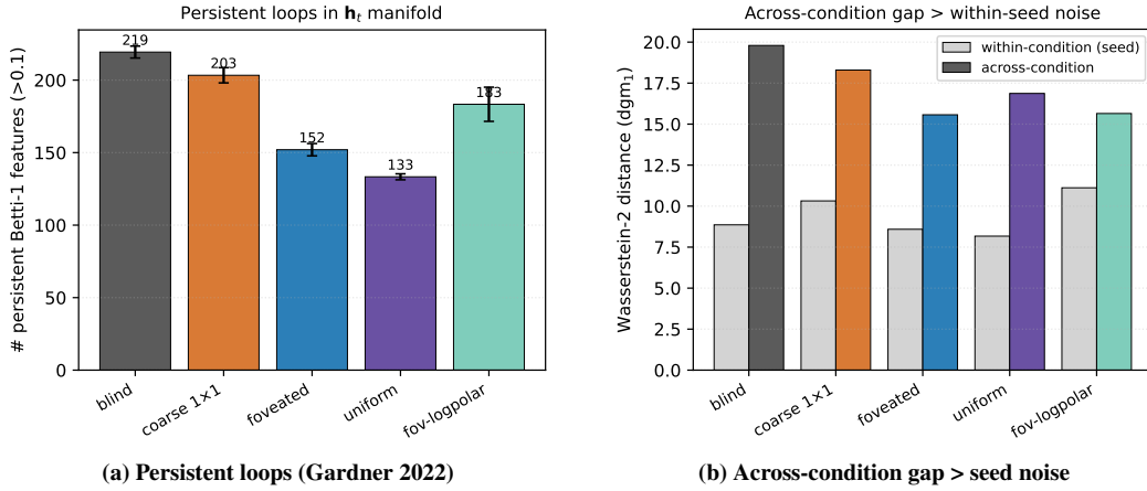
Figure 19: Topological corroboration of the temporal-format dichotomy. (a) Persistent-loop counts (number of H_1 features with persistence > 0.1 ) per condition; loops order monotonically with encoder bandwidth (blind highest, uniform lowest). (b) Wasserstein-2 distance between H_1 persistence diagrams: cross-condition gap exceeds within-condition (seed) noise across all five conditions; the \mathbf{h}_t manifolds are topologically distinguishable.
