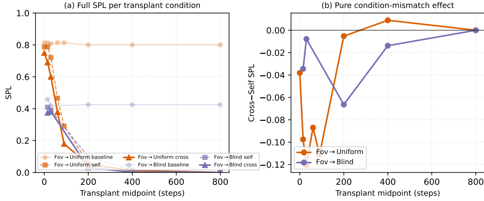
Figure 22: Memory-transplant midpoint sweep. Two representative donor→recipient pairs (foveated→uniform, foveated→blind) across midpoints \{0, 15, 30, 60, 90, 200, 400, 800\} time-steps ( n=100\text{--}150 episodes/cell). The full 5 \times 5 matrix in main Figure ?? is the t=30 slice. (a) Full SPL per condition (baseline / self / cross): t=0 collapses to a protocol-noise floor (the diagonal of the main-text matrix is rollout-divergence noise, not condition mismatch); SPL decays for all conditions at t \geq 200 because by then most successful episodes have terminated. (b) Cross-minus-self isolates condition-mismatch alone. The gap peaks in the t \in [30, 90] window — where the agent has integrated history but is not yet committed to a trajectory — and decays toward 0 at t \geq 400 . The t=30 asymmetry is therefore neither a midpoint-specific artefact nor a late-midpoint inflation.
