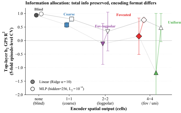
Figure 3: Format shift, not info collapse. Linear (filled, dotted) and 2-layer MLP (hollow, solid) probes per condition; same episode-level 5-fold CV, 20 000 episode-step samples per condition. Linear R^2 range \approx 2.0 across conditions; MLP range \approx 0.5 . Position information is approximately preserved by MLP probing in rich-encoder conditions even when linear readability collapses; MINE-estimated total I(h_2; pos) decreases by only \approx 1.3\times across the same range (Appendix E.4). The remaining variation is in format , the focus of the rest of this section.
