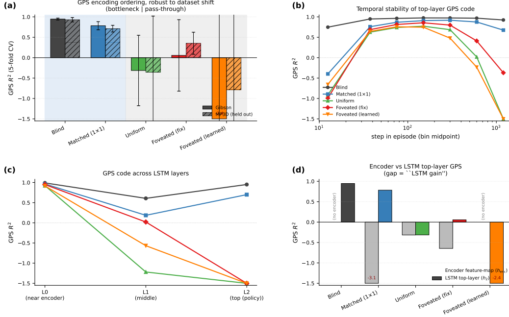
Figure 2: H1 evidence in four panels. (a) Top-layer GPS R^2 (5-fold CV, deterministic rollouts) on Gibson and held-out MP3D (300 episodes/condition). Blind and matched-compute (bottleneck) decode world-frame GPS on both datasets; uniform / foveated / foveated (learned) (rich-encoder) do not, except foveated recovering on MP3D. (b) Top-layer GPS R^2 binned by step-in-episode: all five conditions encode top-layer GPS in the typical window (steps \sim 25 –200); the code becomes no longer linearly readable in the rich-encoder long-tail (negative R^2 in the 800+ step bin), while bottleneck conditions hold R^2 > 0.7 to step 800+. The headline in (a) is therefore primarily long-tail behaviour. (c) Per-LSTM-layer GPS R^2 : all five conditions have GPS at Layer 0 (the GPS sensor embedding enters the LSTM input vector here — a sensor pass-through, not the network “computing” position); divergence is at Layer 2, the policy readout. (d) Encoder feature-map probe (grey bars; post-ResNet-18, pre-LSTM) vs LSTM top-layer probe (coloured bars). Blind and foveated (learned) have no encoder probe (no encoder / no encoder-probe data resp.). The grey bars sit near or below zero everywhere, so no sighted encoder linearly carries GPS ; the coloured-grey gap is the “LSTM gain”. Matched gains \sim 3.9 , uniform \sim 0 , foveated \sim 0.7 .
