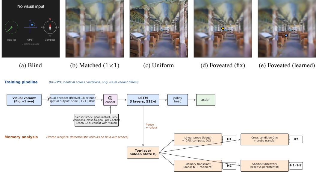
Figure 1: Setup. Top row, (a)–(e) : the five visual sensor conditions, shown on the same scene. (a) Blind : no visual stream; only the non-visual sensor stack. (b) Matched (1x1) : 48x48 uniform RGB, chosen so the ResNet-18 encoder collapses spatially to a 1x1 feature map. (c) Uniform : 256x256 full-resolution RGB. (d) Foveated (fix) : eccentricity-dependent Gaussian blur ( \sigma_{\max} = 8 , quadratic falloff) centred at the image middle (yellow dot). (e) Foveated (learned) : same blur model with a learned (x, y) gaze offset (blue dot, post-training collapsed location (0.49, 0.62)). Bottom block : the structural variable being manipulated is encoder spatial output (none | 1x1 | 8x8); the DD-PPO learner, sensor stack, LSTM backbone, and policy head are otherwise identical. After training, weights are frozen and we collect deterministic rollouts to extract top-layer hidden states h_t , on which we run linear probes (H1 evidence), cross-condition CKA + probe transfer (H2 evidence), memory transplants (H2 behavioural validation), and shortcut discovery (probe-readable vs. policy-used dissociation, §4.5).
