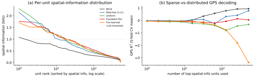
Figure 9: Population coding analysis (referenced from §4.7). (a) Per-unit spatial-information distribution: each curve is one condition’s units sorted by spatial information (descending), x-axis log scale. Counter-intuitively, rich-encoder conditions (uniform / foveated / foveated (learned)) have a few more peaked spatially-tuned units (max \approx 2 bits) than bottleneck conditions; blind has the flattest distribution (max \approx 1 bit, no unit reaches the dashed 1-bit threshold). (b) Sparse-vs-distributed GPS decoding: probe R^2 when only the top- k spatial-info units are used as features. Blind reaches R^2 \approx 1.0 at k = 512 ; matched climbs to R^2 \approx 0.5 ; rich-encoder networks fail to decode GPS at any k even though their top units carry higher per-unit spatial information. The combined picture: higher per-unit spatial information \neq position readout . Rich-encoder peaked units appear to encode features correlated with position (e.g. visual landmarks, trajectory phase) rather than position itself.
