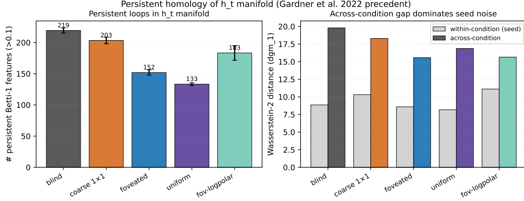
Figure 5: Persistent homology of the recurrent-state manifold (Gardner 2022 [Gardner et al., 2022] precedent). Vietoris–Rips persistence diagrams on 1000-point subsamples of h_t in PCA-32 (cosine distance, 3 seeds per condition; persistence threshold 0.1). Left : persistent Betti-1 (loop) counts. Right : across-condition Wasserstein-2 distance (coloured) compared to within-condition seed-to-seed noise (grey). The across-condition gap is \sim 2\times the within-condition seed noise — conditions are topologically distinguishable. Betti-1 counts order monotonically with encoder bandwidth (in the opposite direction to pre-registration; we report what we found). The clean across-vs-within separation establishes that “the recurrent-state manifold has different topology under different sensors”, a parameter-free format claim that does not depend on the choice of decoder.
