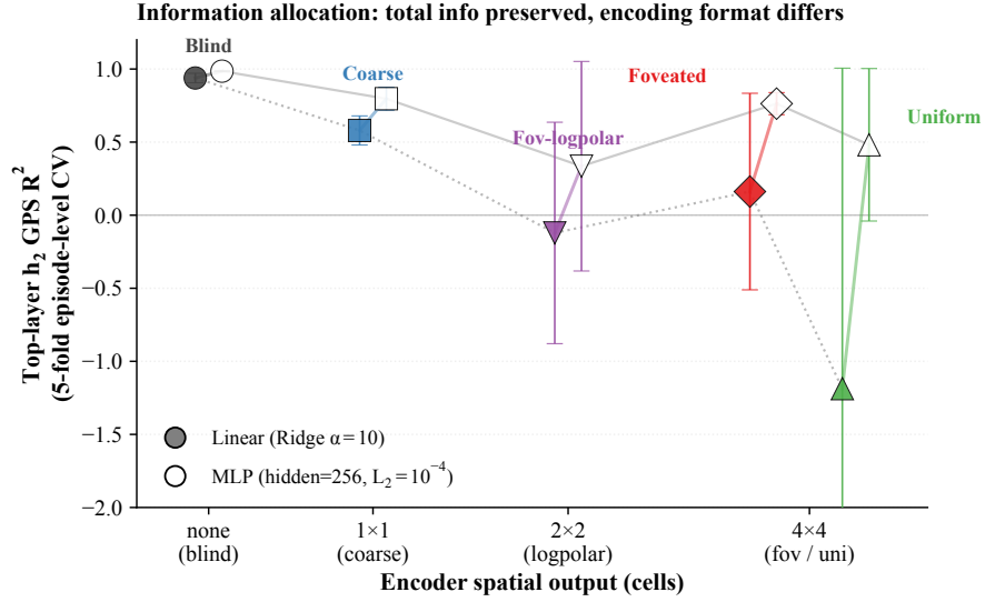
Figure 28: Information allocation: linear vs. MLP readout. Per-condition top-layer h_2 GPS R^2 under linear (filled markers, dotted line) and 2-layer MLP probing (hollow markers, solid line); same episode-level 5-fold CV, 20 000 episode-step samples per condition. Linear R^2 range \approx 2.0 across conditions; MLP range \approx 0.5 . Position information is approximately preserved by MLP probing in rich-encoder conditions even when linear readability collapses — a format shift, not a total-information collapse. MINE-estimated total I(h_2; \text{pos}) shows a more modest \approx 1.3\times decrease across conditions (Appendix E.4).
