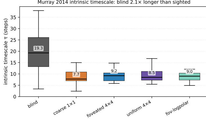
Figure 4: Murray 2014 intrinsic timescale: the blind agent integrates \sim 2.1\times longer than any sighted condition. Per-unit single-exponential autocorrelation-decay \tau on PCA-30-reduced \mathbf{h}_t , 30 units per condition, fit R^2 > 0.5 kept. Boxes: IQR; whiskers: P10–P90 of fitted \tau . The BLIND median \tau=19.3 steps lies above the 90th percentile of every sighted condition. Method follows Murray et al. 2014 [Murray et al., 2014] and re-runs their cortical-hierarchy fast-sensor / slow-integrator dichotomy on a recurrent navigator: the encoder-bandwidth axis does the same job here.
