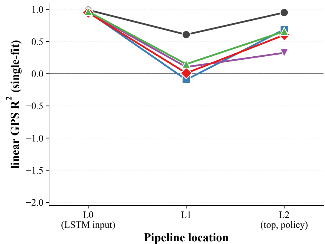
(c) Pipeline view: where the divergence sits
