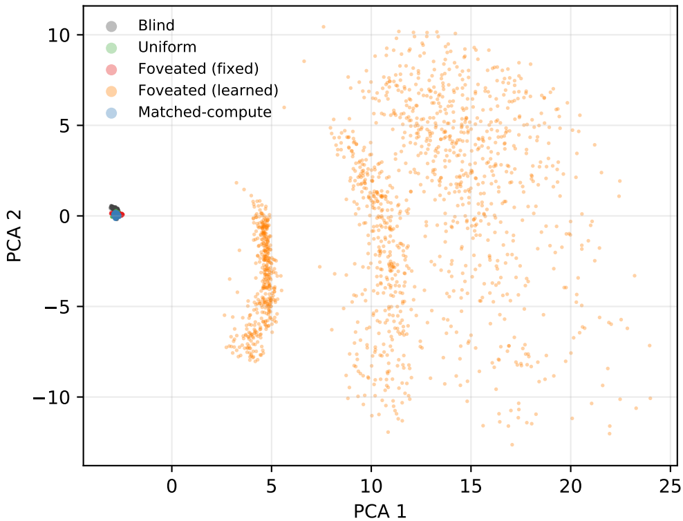
Hidden-state geometry across conditions (PCA)
