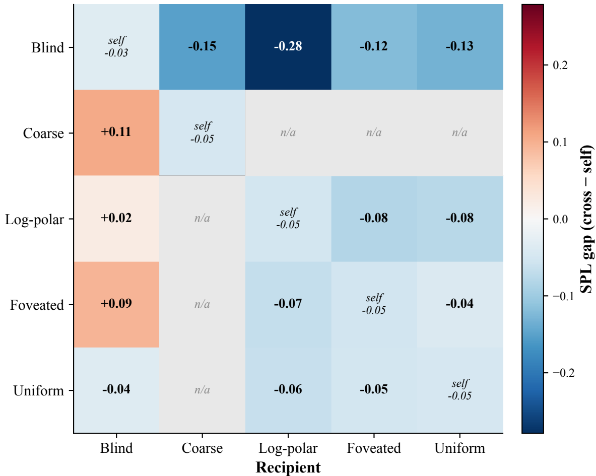
Cross-condition memory transplants
