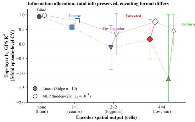
Figure 3: Format shift, not information collapse. Linear (filled) and 2-layer MLP (hollow) probes per condition. Linear R^2 varies widely across conditions; MLP R^2 is preserved. The remaining variation is in format .
