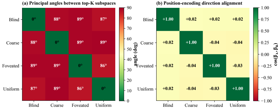
Figure 6: Subspace divergence: conditions occupy mostly-orthogonal subspaces of h_2 . (a) Mean principal angles between top- K PCA subspaces (close to orthogonal across all condition pairs). (b) Pairwise cosines between Ridge-probe position-directions (near zero). Position is encoded along essentially uncorrelated directions across conditions.
