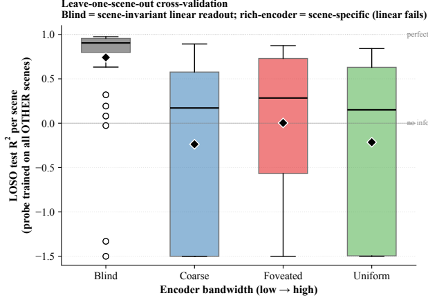
Figure 4: LOSO cross-validation: only blind’s linear position readout generalises across scenes. Ridge probe trained on \sim 30 Gibson scenes, tested on the held-out scene; box plot per condition. Bottleneck conditions force a scene-invariant position-direction; rich encoders induce scene-conditional encoding that a single linear probe cannot capture.
