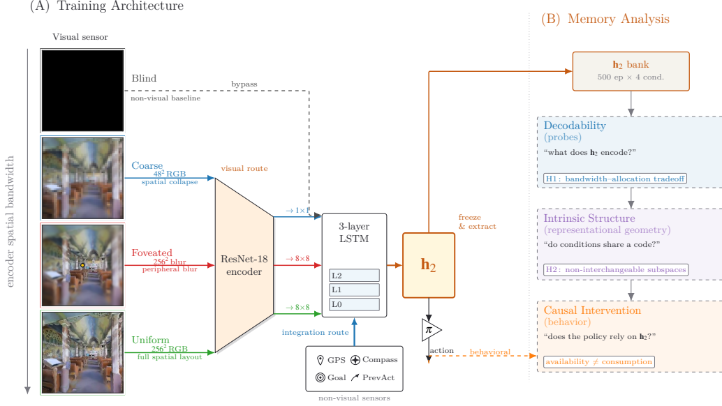
Figure 1: Experimental setup and analysis pipeline. Row 1 (architecture): four sensor conditions span an axis of encoder spatial bandwidth ( blind, coarse, foveated, uniform ; leftmost column), feeding a shared ResNet-18 encoder + 3-layer LSTM; blind bypasses the encoder. A log-polar foveation control (Appendix G) adds a 5th intermediate point on the same axis. Row 2 (analysis): three method blocks — decodability, intrinsic structure, causal intervention — read the frozen top-layer hidden state h_2 \in \mathbb{R}^{512} to test three axes of one capacity allocation: magnitude, format, consumption (§2; synthesis in §4).
