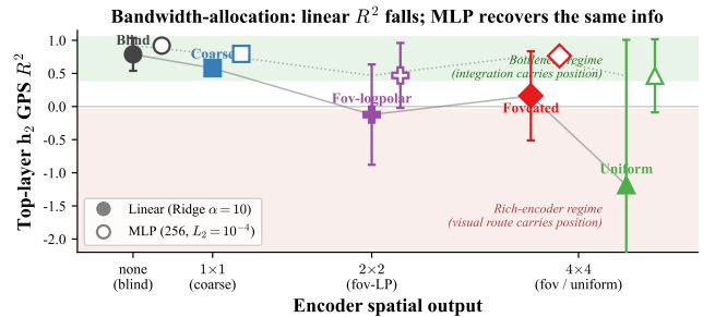
Figure 1. Top-layer GPS R^2 (mean \pm \sigma ) vs. encoder spatial output. Solid: linear (Ridge) probe. Dashed: 2-layer MLP probe on the same hidden states. Blind point: preliminary 100-ep partial NPZ.
