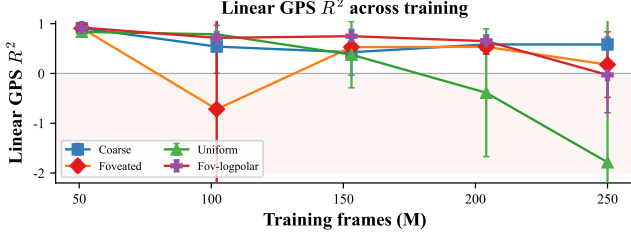
Figure 2. Linear GPS R^2 at 5 training checkpoints per sighted condition. The blind cross-training trajectory is deferred to the final report (intermediate blind checkpoints exist but have not yet been re-probed under the unified pipeline). Negative- R^2 outliers clipped to -2.0 .
