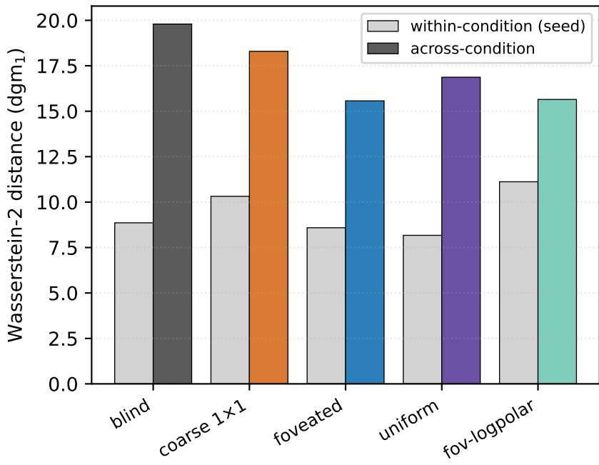
Across-condition gap > within-seed noise
