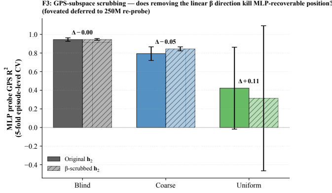
Figure 18: \beta -subspace scrubbing. For each cond (foveated deferred), Ridge \beta identifies a 2-d direction in \mathbf{h}_2 that linearly predicts (x, y); scrubbed \mathbf{h}_2 = (I - \beta^+ \beta) \mathbf{h}_2 removes this 2-d subspace. MLP probe is essentially unaffected by scrubbing across all three conditions: position information is redundantly distributed across many \mathbf{h}_2 dimensions, not concentrated in the 2-d \beta subspace.
