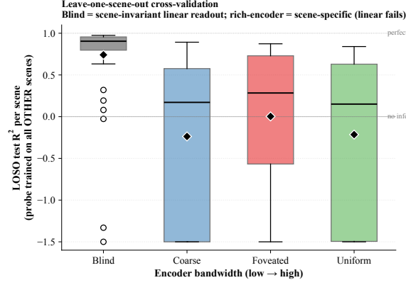
Figure 24: Leave-one-scene-out (LOSO) cross-validation. For each cond, Ridge probe trained on \sim 30 Gibson scenes (top scenes by sample count) and tested on the held-out scene. Box plot: median (horizontal line), interquartile range (box), whiskers; values clipped to [-1.5, 1] for visualisation. Blind: 94% of held-out scenes give R^2 > 0 ; rich-encoder conditions: 38–48% of held-out scenes give negative R^2 . Encoder bandwidth dictates whether the linear position-axis is scene-invariant (linearly probable across scenes) or scene-conditional (requires non-linear readout to switch contexts).
