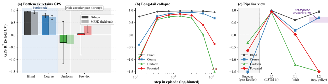
Figure 26: Magnitude-axis evidence in detail. (a) Top-layer GPS R^2 on Gibson and held-out MP3D (5-fold CV, deterministic rollouts, 300 ep/cond; lighter bars = MP3D; values outside y-range labelled). (b) Top-layer GPS R^2 binned by step-in-episode (7 log-spaced bins in [10, 1600+] , right-most bin pools \geq 1024 ). (c) GPS R^2 along Encoder \rightarrow L0 (sensor concat) \rightarrow L1 \rightarrow L2 (policy-readable). Shaded band at L2: 2-layer MLP probe recovery range ( R^2 \in [0.51, 0.73] ). Blind has no encoder.
