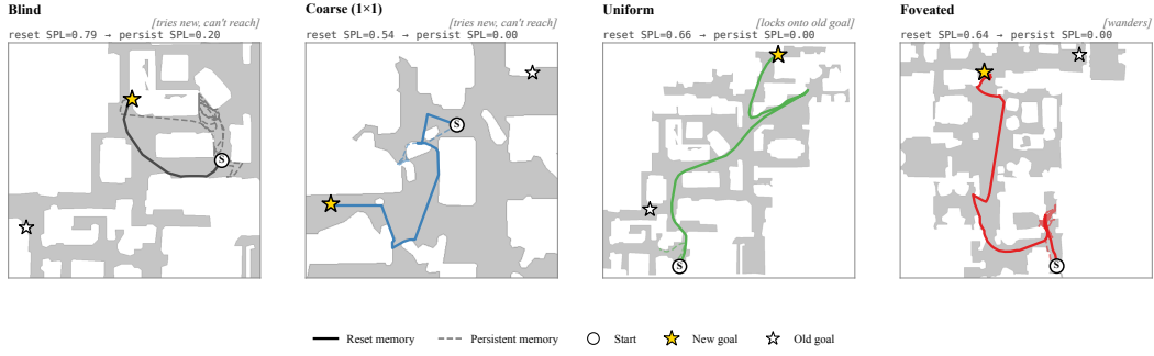
Figure 31: Persistent-memory failure modes — one canonical paired-episode case per condition (extended catalog: Appendix E.6). Aggregate per-condition margin = avg dist(persistent end → old goal) − avg dist(persistent end → new goal) over same-floor failures (reset SPL > 0.5, persistent SPL < 0.2, persistent steps ≥ 30, |\Delta y_{\text{goal}}| < 0.5\text{m} ): Blind −0.38m ( n=27 ), Coarse −0.57m ( n=35 ), Foveated −0.59m ( n=16 ), Uniform +1.83m ( n=46 , closer to OLD goal) . Single seed.
