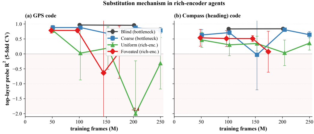
Figure 27: Cross-training probe profile across 4–5 training checkpoints per condition, truncated at 250M frames. (a) Top-layer GPS R^2 . (b) Top-layer compass R^2 . (500 ep/probe, 5-fold CV, single seed; hollow dotted = partial-data ckpts; negative- R^2 outliers clipped at -2.0 .)
