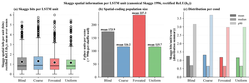
Figure 28: Skaggs spatial information per LSTM unit. (a) Distribution of per-unit Skaggs bits (averaged across 15 top scenes per condition); bottleneck and rich-encoder conditions overlap substantially (means \approx 1.16 – 1.32 bits). (b) Number of place units per scene exceeding the 99th percentile of a 100-shuffle null; foveated has the largest count ( \approx 237 /scene), blind/coarse/uniform \approx 116 – 174 . (c) Distribution summary; cross-condition differences sit within the within-condition spread. The canonical Skaggs metric on rectified activations does not by itself discriminate bottleneck from rich-encoder regimes.
