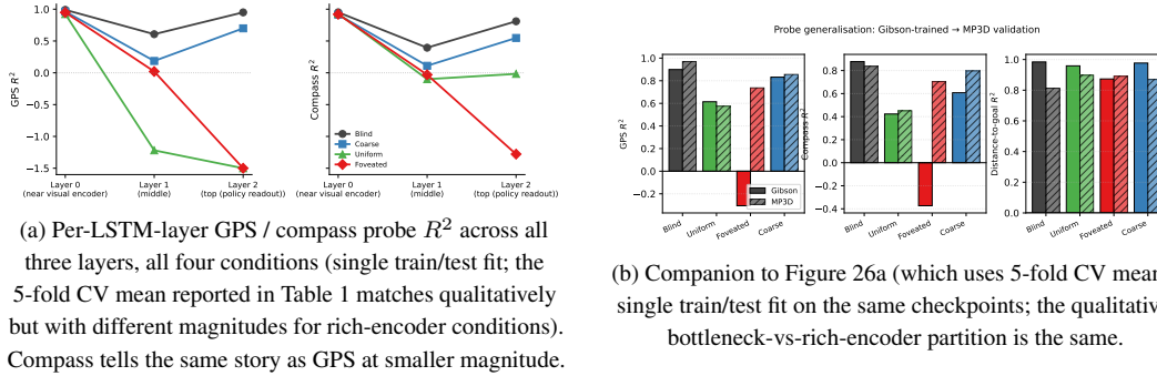
Figure 22: Per-layer and MP3D companion figures (referenced from §3.2).
