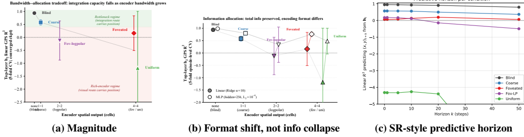
Figure 2: The capacity-allocation principle: three converging signatures of bandwidth \rightarrow format shift. (a) Magnitude . Top-layer h_2 linear GPS R^2 (5-fold CV, mean \pm \sigma ) vs. encoder spatial output dimension. The monotonic anti-correlation is the bandwidth–allocation tradeoff: as encoder spatial bandwidth grows, less integration capacity remains in the recurrent state. Foveated and uniform share x but differ in y , showing the design space is not 1-D — channel-level information is a second axis (Appendix G). (b) Format shift, not info collapse . Linear (filled, dotted) and 2-layer MLP (hollow, solid) probes per condition. Linear R^2 range \approx 2.0 across conditions; MLP range \approx 0.5 . Position information is approximately preserved by MLP probing where linear readability collapses — a format shift, not a total-information loss. MINE-estimated total I(h_2; \text{pos}) shows only a \approx 1.3\times shift across the same range (Appendix E.4). Since the DD-PPO action head is a linear projection of h_2 , “linearly decodable at L2” = “policy-accessible”. (c) Predictive horizon (Stachenfeld 2017 SR-style cognitive-map signature) . Linear R^2 predicting future position (x, y)_{t+k} from h_t vs. horizon k . BLIND retains R^2 \geq 0.90 to k=20 and +0.79 at k=50 ; COARSE a moderate R^2 \in [0.50, 0.57] to k=20 ( +0.37 at k=50 ); rich-encoder conditions show no predictive horizon (foveated stays in [0.06, 0.19] flat, foveated-logpolar turns negative by k=20 , uniform is strongly negative throughout). Blind’s h_t encodes future-state occupancy, the SR-style cognitive-map signature; rich-encoder h_t does not extrapolate temporally even with non-linear flexibility. All panels use 500 Gibson held-out episodes per condition (5-fold CV; blind at 340M frames, sighted at 250M; Appendix A).
