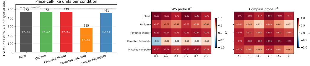
Figure 6: [Stochastic-collection data; regeneration from deterministic probes pending.] Left : LSTM units with > 1 bit spatial information per condition [Banino et al., 2018]; mean bits \bar{s} shown inside bars. Right : Per-layer, per-state linear probe R^2 for GPS (left sub-panel) and compass (right sub-panel). The qualitative pattern — broad per-unit spatial encoding in most conditions, with foveated-learned an outlier, and the heading- \rightarrow -position dissociation preserved across layers — is the load-bearing claim. The specific unit counts and per-layer R^2 values were computed on pre-fix stochastic rollouts (see §3.3); the deterministic re-run will update the numbers and, under the new H1 framing, we expect the broad-encoding/layer-invariance qualitative pattern to hold while the absolute R^2 values rescale toward the current-state numbers in Table 1.
