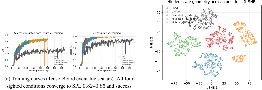
(b) [Stochastic-collection data; regeneration pending.] t-SNE projection of top-layer LSTM hidden states pooled across all five conditions (perplexity 30). The five conditions occupy non-overlapping regions of the 2-D embedding — a visual confirmation of the near-zero CKA result (§4.3). Computed on pre-fix stochastic rollouts; deterministic re-run will regenerate.
