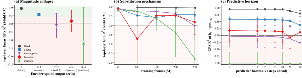
Figure 2: Three views of the magnitude axis. (a) How much linearly-readable position survives at the policy-readable layer, plotted against encoder bandwidth: more visual bandwidth means less of the integrated GPS code remains linearly accessible. (b) When the divergence appears: rich-encoder conditions start with the same high readability as bottleneck conditions and then lose it over training, while bottleneck conditions hold the code throughout. (c) How far into the future the hidden state predicts position: at increasing lags k , only the bottleneck conditions still encode where the agent is heading; rich-encoder hidden states carry no forward-rollout structure. Together, (a)–(c) place the magnitude collapse on three independent axes: cross-condition, across-training, and across the planning horizon.
