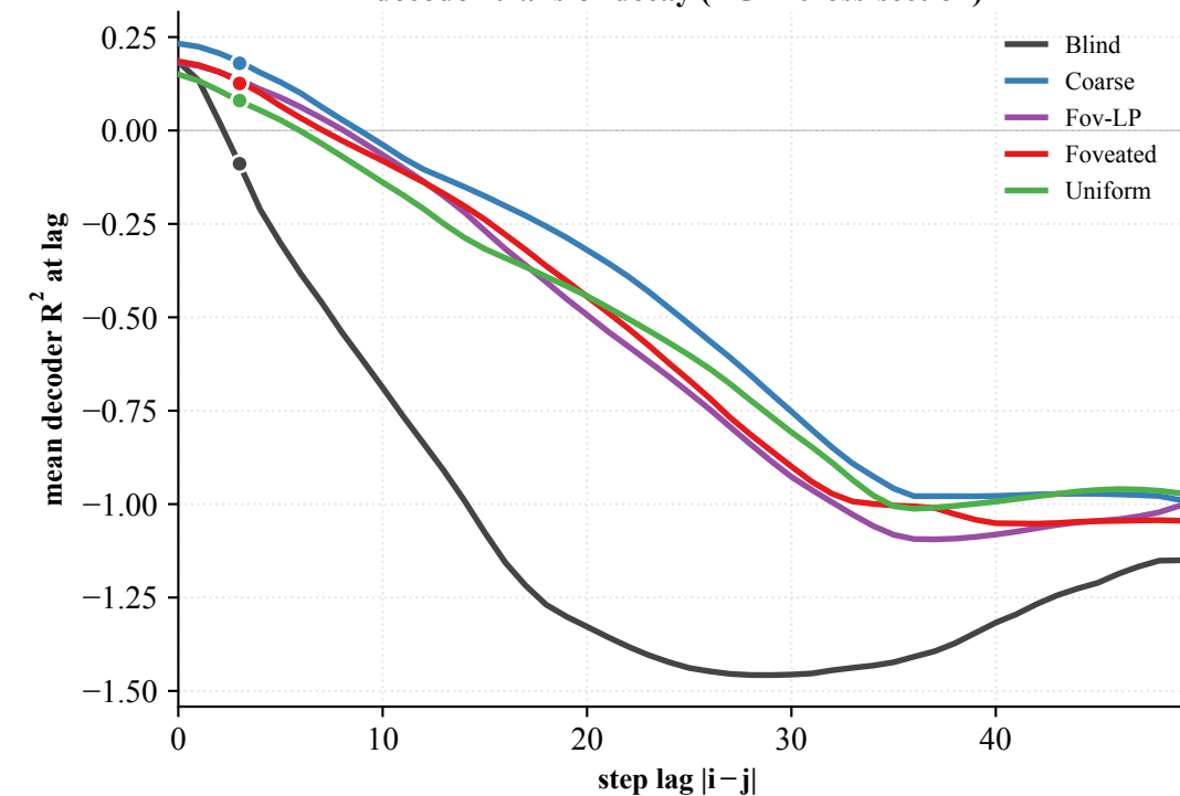
decoder-transfer decay (TGM cross-section)
