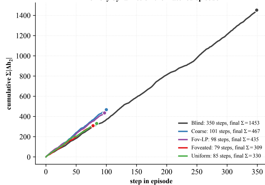
memory dynamics on the matched episode
