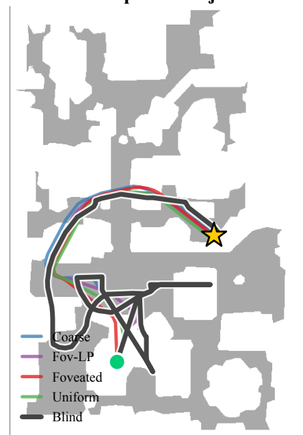
matched-episode trajectories
