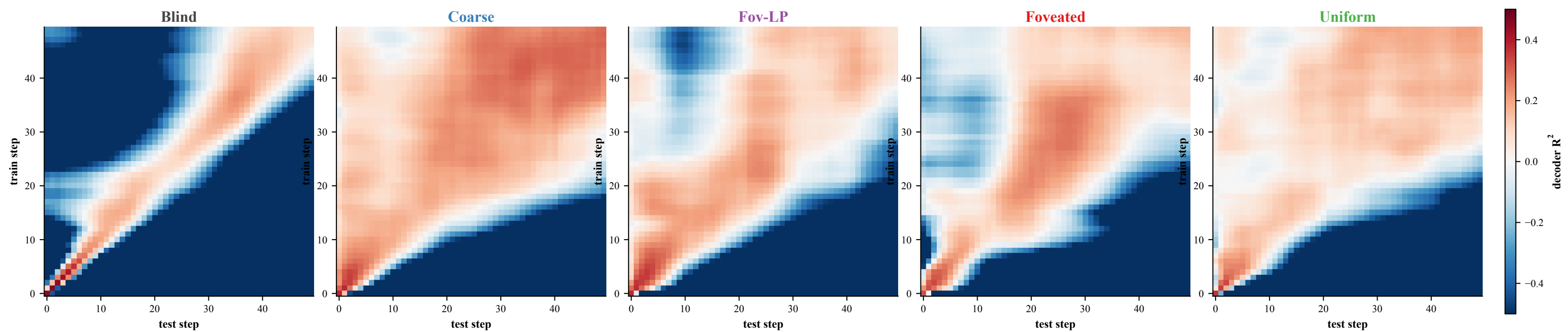
matched-episode trajectories
