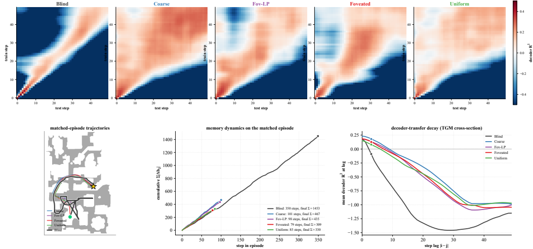
Figure 4: Temporal format: four complementary views of the same dichotomy and within-sighted spectrum. Top row: step-by-step generalisation of a linear goal-vector decoder. Each 50 \times 50 heatmap shows decoder R^2 when fit at step i (row) and evaluated at step j (column). A diagonal-only structure (blind) signals a step-by-step rotating basis: the decoder at step t does not transfer to step t \pm 30 . A square-block structure (coarse) signals a stationary readout. Sighted-rich conditions interpolate. Bottom row, left: matched-episode trajectory overlay (Almena, episode 157; same start = green disc, same goal = yellow star). The four sighted paths bundle into a single direct corridor route (79–101 steps); blind winds for 350 steps. Middle: cumulative memory displacement \Sigma|\Delta \mathbf{h}_2| vs step-in-episode, one curve per condition. Blind’s curve ends at 1453 over 350 steps; sighted conditions stop early at 309–467 (foveated 309 < uniform 330 < fov-LP 435 < coarse 467). Right: mean decoder R^2 as a function of step lag |i - j| — each top-row TGM heatmap collapsed to a single curve. The five curves fan out monotonically: blind drops to \approx -1.2 (catastrophic transfer); coarse holds R^2 \approx +0.18 at small lag (strongest stationary block); fov-LP +0.13 , foveated +0.13 , uniform +0.08 . The within-sighted ranking inverts encoder bandwidth: less bandwidth, more stationary readout. Per-unit autocorrelation \tau values (Murray [Murray et al., 2014]) and a persistent-homology corroboration [Gardner et al., 2022] are reported in Appendix F.
