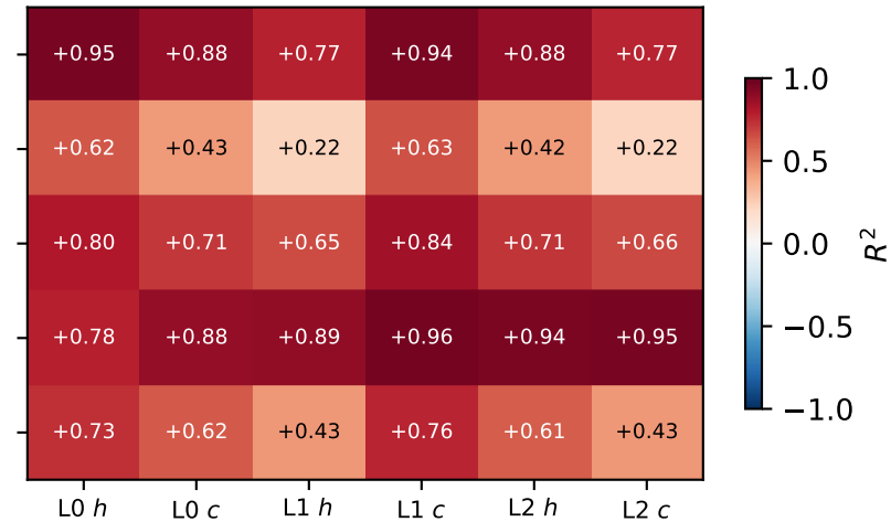
Compass probe R^2
