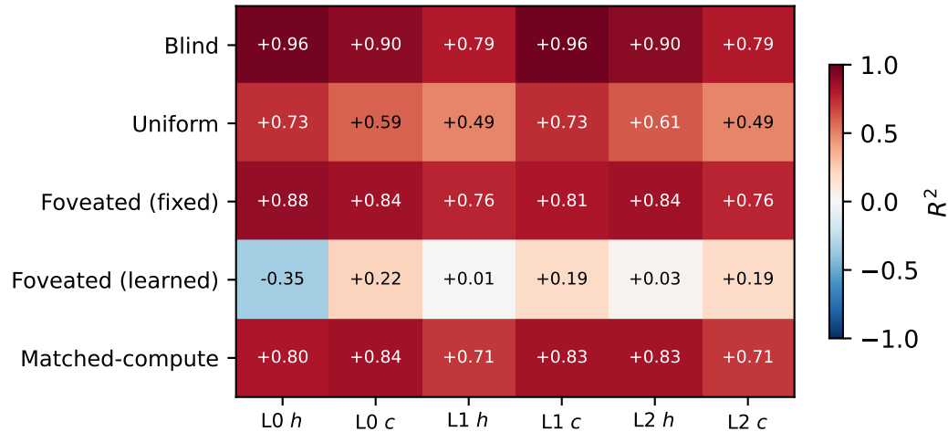
GPS probe R^2
