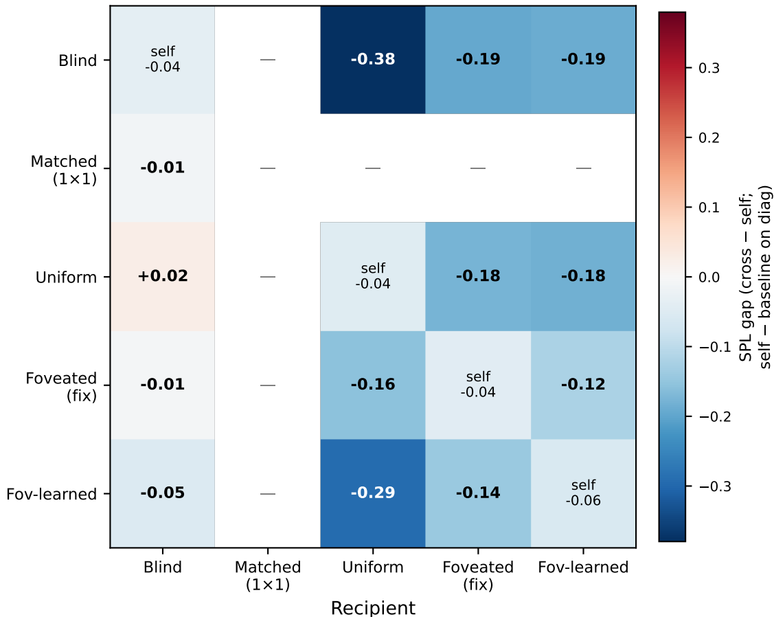
5×5 cross-condition transplant matrix (midpoint = 30 steps; isolated condition-mismatch effect)
