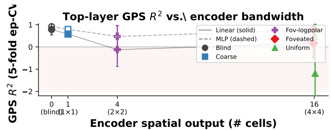
Figure 1. Top-layer GPS R^2 (mean \pm \sigma ) vs. encoder spatial output. Solid: linear (Ridge) probe. Dashed: 2-layer MLP probe on the same hidden states. Blind point: preliminary 100-ep partial NPZ.
