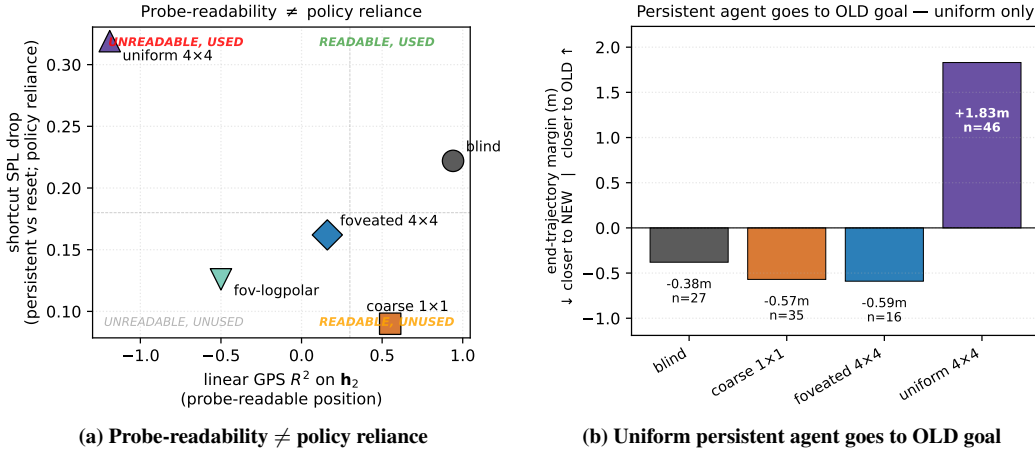
Figure 9: Consumption-axis dissociation: probe-readable position is not what drives behaviour. (a) Off-diagonal cases . Per-condition shortcut SPL drop (persistent vs reset LSTM, paired same-scene-different-goal episodes; y -axis = policy reliance) plotted against linear GPS R^2 on \mathbf{h}_2 ( x -axis = probe-readable position). Two off-diagonal conditions break the assumed probe→policy mapping: COARSE sits in “READABLE–UNUSED” (linear GPS available but ignored by policy), UNIFORM in “UNREADABLE–USED” (no linear GPS yet largest behavioural reliance on persistent memory). (b) The substitute uniform reads . End-trajectory margin = avg dist(persistent end \rightarrow old goal) – avg dist(persistent end \rightarrow new goal) on same-floor failures (reset SPL > 0.5 , persistent SPL < 0.2 , persistent steps \geq 30 , |\Delta y_{\text{goal}}| < 0.5 m). Negative = closer to NEW goal; positive = closer to OLD goal. Only UNIFORM ends closer to the previous episode’s goal (+1.83m, n=46 ); BLIND, COARSE, FOVEATED all end closer to the new goal (−0.38 to −0.59m). The substitute is a visual / scene-history anchor: “head to where you were going last episode.” Canonical per-condition trajectory examples: Figure 35; full 4×4 catalog: Appendix E.6.
