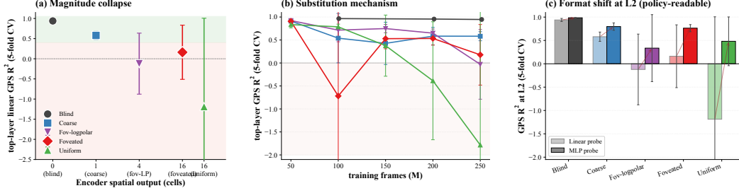
Figure 2: Capacity allocation along the magnitude axis. (a) Linear GPS R^2 at h_2 falls monotonically with encoder bandwidth (5-fold CV; foveated-logpolar at \sim 2 \times 2 lands in the rich regime). (b) The collapse develops over training only for rich-encoder conditions; bottleneck conditions hold the linear code throughout. (c) The cross-condition divergence sits at L2 (policy-readable layer), not at the encoder or LSTM input; star markers show that an MLP probe still reads position at L2 — the linear \rightarrow MLP gap is the format shift quantified in §3.2. Post-retrain hp-consistent agents (Appendix A); panel-level detail in Appendix Figures 30, 31, 32.
