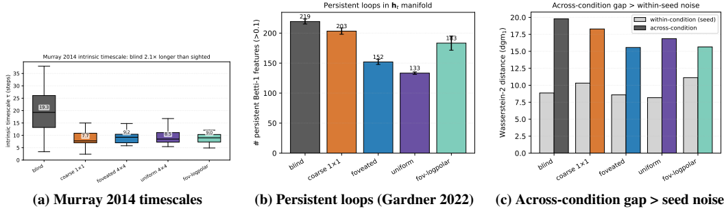
Figure 8: Three independent cogneuro metrics converge on the blind-vs-sighted dichotomy (companion to TGM in Fig. 7). (a) Murray 2014 intrinsic timescales . Per-unit single-exponential autocorrelation-decay \tau on PCA-30-reduced \mathbf{h}_t , 30 units per condition, fit R^2 > 0.5 kept. Boxes: IQR; whiskers: P10–P90 of fitted \tau . The BLIND median \tau=19.3 lies above the 90th percentile of every sighted condition. The encoder-bandwidth axis reproduces Murray et al. 2014 [Murray et al., 2014]’s cortical-hierarchy fast-sensor / slow-integrator dichotomy. (b) Persistent Betti-1 counts (Gardner 2022 [Gardner et al., 2022] precedent). Vietoris–Rips persistence diagrams on 1000-point \mathbf{h}_t subsamples (PCA-32 cosine distance, 3 seeds, persistence threshold 0.1). Loop counts order monotonically with encoder bandwidth (opposite direction from pre-registration; we report what we found). Mechanistic reading: blind path-integration revisits aliased states under sensory degeneracy, creating short-lived loops; uniform’s visual signal tags each location uniquely, producing a tree-like manifold with fewer cycles. (c) Across-condition Wasserstein-2 ( dgm_1 ) gap dominates within-condition seed noise . Mean across-pair distance \approx 17.6 , mean within-condition seed-to-seed \approx 9.4 ; conditions are topologically distinguishable, a parameter-free format claim independent of any probe choice.
