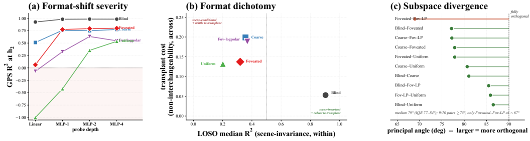
Figure 3: Three views of spatial format. (a) Linearity (probe-depth sweep) : GPS R^2 vs probe depth (linear \rightarrow MLP-1 \rightarrow MLP-2 \rightarrow MLP-4). Blind is essentially fully linear; coarse intermediate; rich-encoder conditions heavily non-linear, depth required growing with encoder bandwidth. (b) Scene-context dependence : LOSO R^2 on x (single-axis transfer across rooms); cross-condition memory-transplant cost on y . Blind sits alone in the scene-invariant + transplant-robust quadrant; the four sighted conditions cluster in the scene-conditional + transplant-brittle quadrant. (c) Subspace divergence : principal angle between every pair of conditions’ position-direction subspaces. 9/10 pairs at \geq 75^\circ ; only the foveated/foveated-logpolar pair at \sim 67^\circ .
