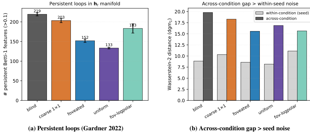
Figure 24: Topological corroboration of the temporal-format dichotomy. (a) Persistent-loop counts (number of H_1 features with persistence > 0.1 ) per condition; loops order monotonically with encoder bandwidth (blind highest, uniform lowest). (b) Wasserstein-2 distance between H_1 persistence diagrams: cross-condition gap exceeds within-condition (seed) noise across all five conditions; the \mathbf{h}_t manifolds are topologically distinguishable.
