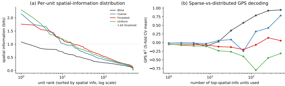
Figure 16: Population-coding analysis: per-unit spatial information vs. population readout. (a) Per-unit spatial-information distribution per condition (units sorted by spatial information, descending; \log x ). Rich-encoder conditions (uniform, foveated) have a few more peaked spatially-tuned units (max \approx 2 bits) than bottleneck conditions; blind has the flattest distribution (max \approx 1 bit). (b) Sparse-vs-distributed GPS decoding: probe R^2 when only the top- k spatial-info units are used as features. Blind reaches R^2 \approx 1.0 at k=512 ; coarse climbs to R^2 \approx 0.5 ; rich-encoder networks fail to decode GPS at any k even though their top units carry higher per-unit spatial information. The picture is: higher per-unit spatial information \neq population position readout. Rich-encoder peaked units encode features correlated with position (visual landmarks, trajectory phase) rather than position itself. Cache: 4 conditions; fov-LP omitted as in §D.
