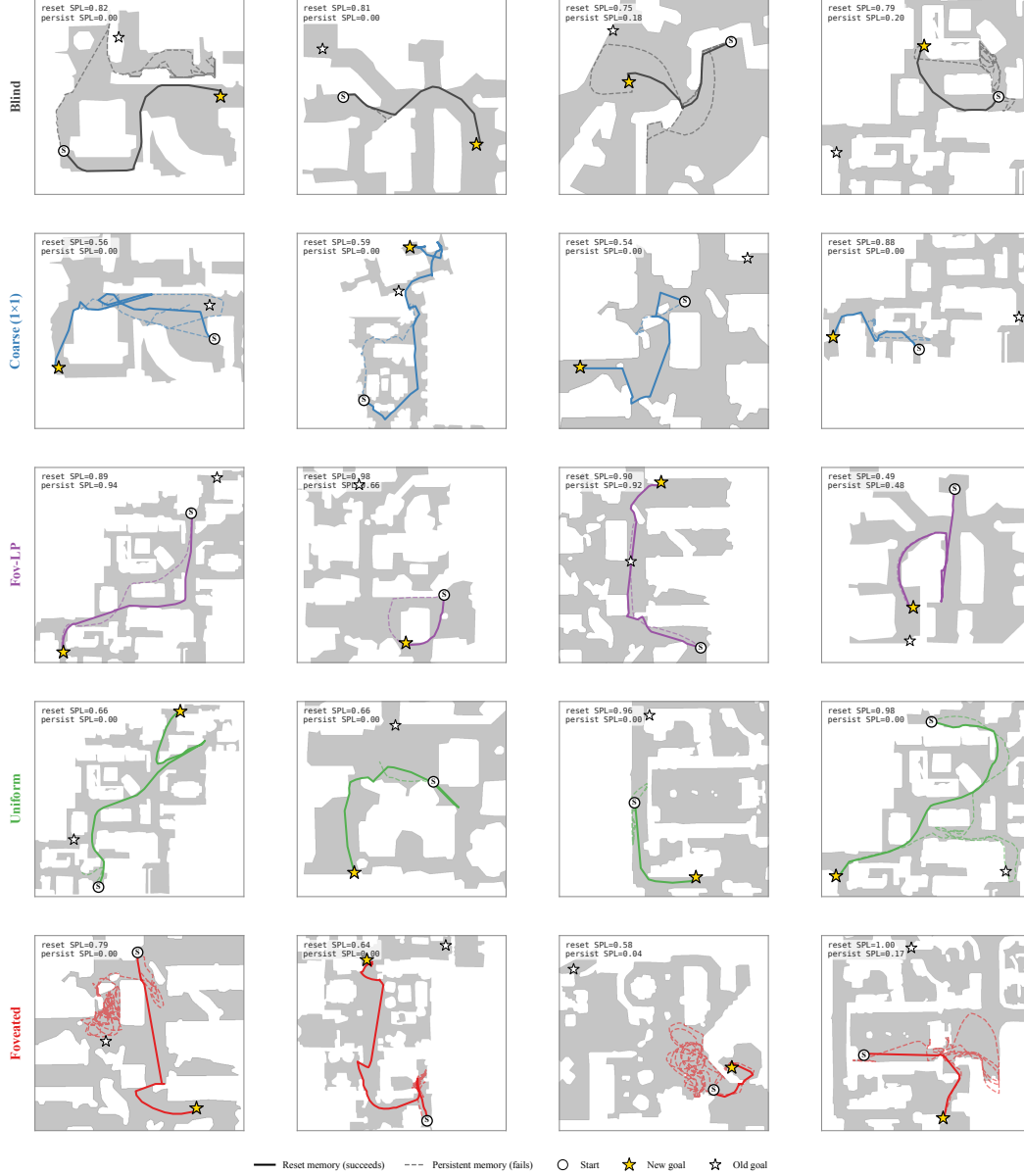
Figure 26: Persistent-memory failure-mode catalog: 4 cases per condition spanning the per-condition margin distribution. Reset trajectory (solid, condition colour) reaches the new goal; persistent trajectory (dashed bold) shows where the persistent-memory agent ends up. Bottleneck conditions (Blind, Coarse) cluster at “tries-new”; Fov-LP also tries-new in all four selected cases (its persistent agent rarely fails to reach the new goal, the “robust to memory carryover” pattern); Uniform clusters at “locks-onto-old”; Foveated is mixed.
