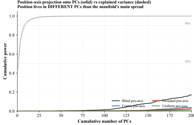
Figure 19: Position-axis lives in low-variance directions of h_2 . Solid: cumulative power of the Ridge-probe singular directions (the linear position-axis) as a function of # PCs. Dashed: cumulative explained variance (the manifold’s own variance distribution). The manifold’s variance is concentrated in \sim 7 –9 top PCs (90% by PC 9), but the position-axis distributes its power across 200+ PCs — it does not reach 50% within the first 200 PCs. Position information is encoded in the low-variance tail of h_2 across all conditions; the discriminator across conditions is therefore not where (in a high-variance sense) position lives but rather the cross-scene stability of the readout direction (Figure 3b). Cache: 4 conditions; fov-LP omitted as in gD.
