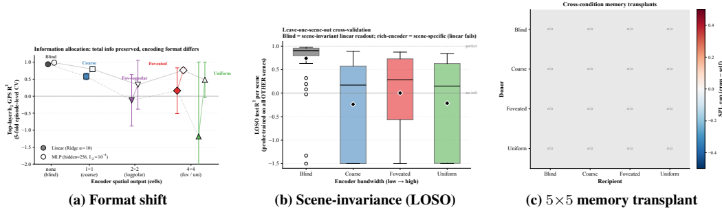
Figure 3: Three views of the format axis. (a) Format shift : linear (filled) and 2-layer MLP (hollow) probes per condition. Linear R^2 varies widely; MLP R^2 is preserved — a format shift, not an information loss. (b) Scene-invariance (LOSO) : Ridge probe trained on \sim 30 Gibson scenes, tested on the held-out scene. Only blind’s linear readout generalises; rich encoders induce scene-conditional encoding. (c) Memory transplant : 5 \times 5 cross-condition matrix at midpoint t=30 . Direction-asymmetric: bottleneck \rightarrow rich-encoder transplant breaks the recipient; rich-encoder \rightarrow bottleneck preserves it.
