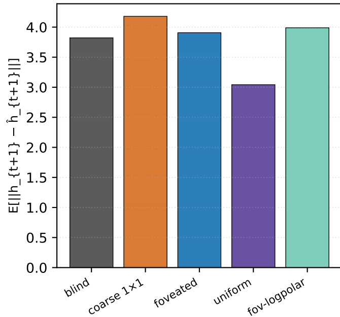
Mean prediction-error magnitude
