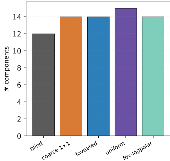
Residual cov rank (90% var)
