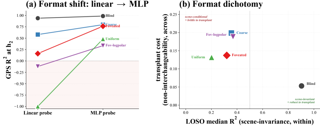
Figure 3: Two views of the format axis. (a) Format shift : slope chart from Linear to MLP probe per condition; steep slope = large gap between linear and non-linear readability. Bottleneck conditions sit on near-horizontal slopes; rich-encoder conditions on near-vertical ones — a format shift, not an information loss. (b) Format dichotomy : LOSO median R^2 (within-condition scene-invariance) vs. mean cross-condition transplant cost (across-condition non-interchangeability). Bottleneck (blind) sits in the scene-invariant + transplant-robust quadrant; rich-encoder conditions cluster in the scene-conditional + transplant-brittle quadrant. (Coarse n=1 cross-pair — differing input size excludes it from most pairs.)
