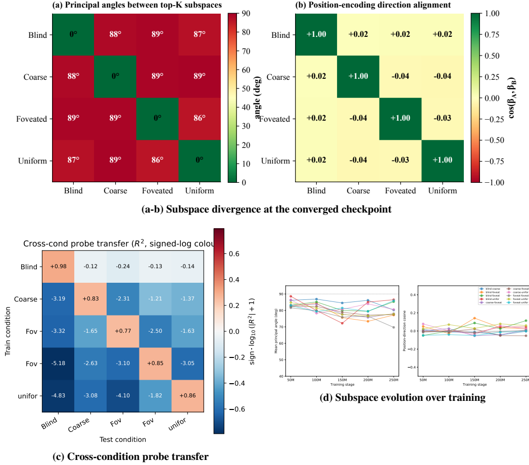
Figure 28: Format axis: corroborating diagnostics (referenced from §3.2). (a) Principal angles between top- K PCA subspaces of \mathbf{h}_2 : close to orthogonal across all condition pairs. (b) Pairwise cosines between Ridge-probe GPS-direction weights: near zero. (c) Cross-condition probe transfer matrix (train on row, test on column): off-diagonal R^2 is catastrophically negative — the position-axes encoded across conditions are jointly incompatible at the readout level. (d) Subspace divergence is established early: principal angles are already near-orthogonal at the earliest probed checkpoint ( \sim 50 M frames) and stay so throughout, indicating the structural separation is laid down well before convergence.
