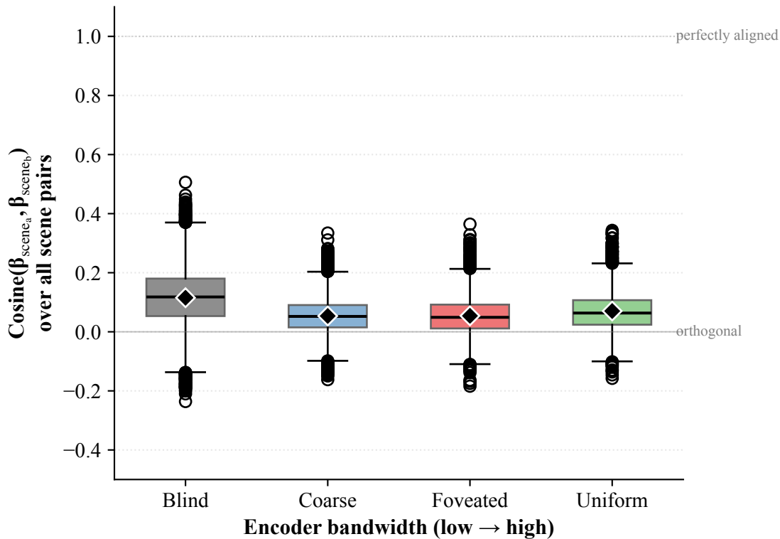
Per-scene position-direction stability across conditions (higher = same readout works across scenes; lower = scene-specific encoding)
