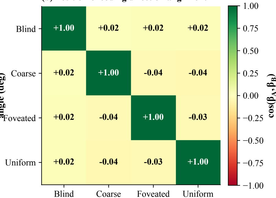
(b) Position-encoding direction alignment
