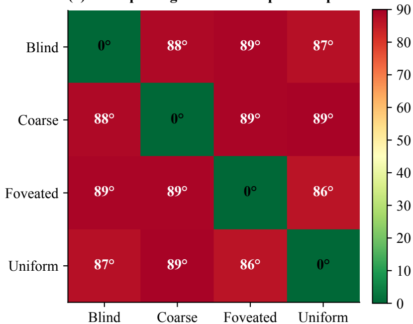
(a) Principal angles between top-K subspaces
