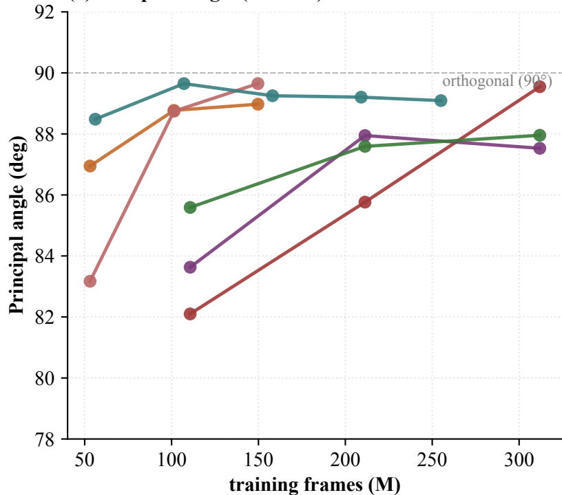
(a) Subspace angle (zoomed)
