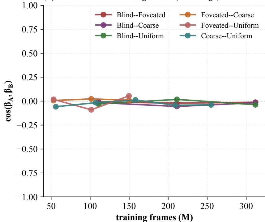
(b) Position-direction alignment (full range)
