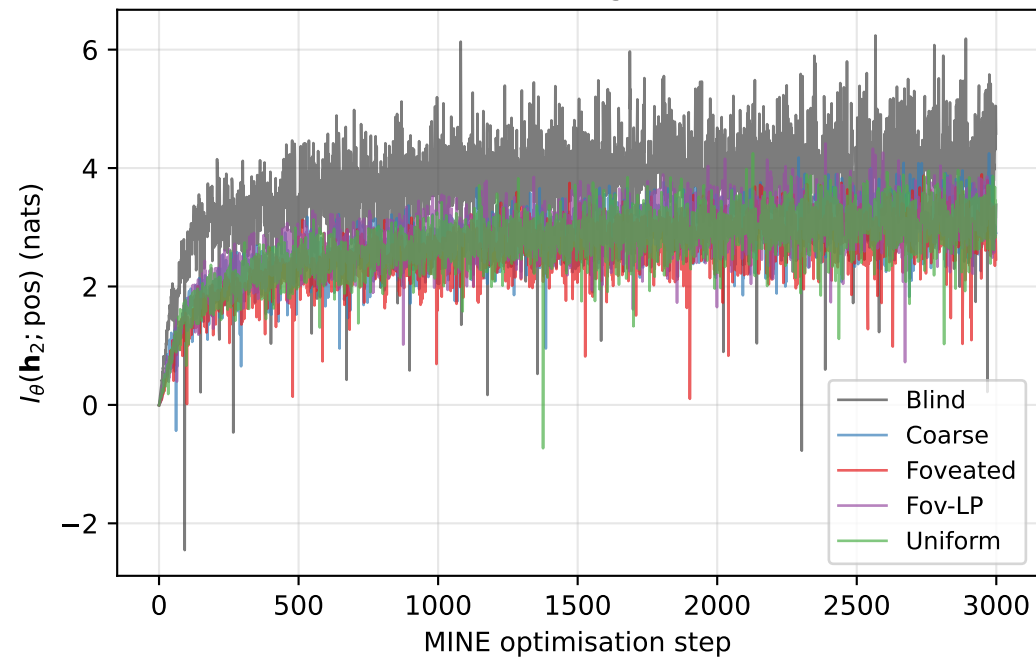
MINE training curves
