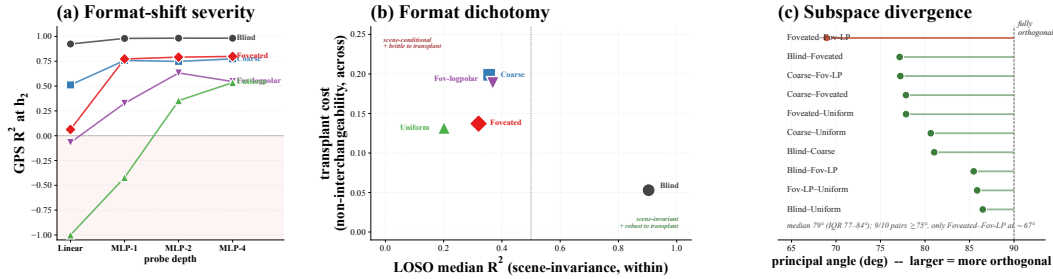
Figure 3: Three views of spatial format. (a) Linearity (probe-depth sweep) : GPS R^2 vs probe depth (linear \rightarrow MLP-1 \rightarrow MLP-2 \rightarrow MLP-4) per condition. Blind’s code is essentially fully linear (depth recovers nothing new); coarse is intermediate; the three rich-encoder conditions are heavily non-linear, with the depth required to recover position growing with encoder bandwidth. (b) Scene-context dependence : leave-one-scene-out R^2 on x (does a single linear axis transfer across rooms?); cross-condition memory-transplant cost on y (does foreign memory drive my policy?). Blind sits alone in the scene-invariant + transplant-robust quadrant; the four sighted conditions cluster in the scene-conditional + transplant-brittle quadrant. (c) Subspace divergence : principal angle between every pair of conditions’ position-direction subspaces, sorted high-to-low. 9/10 pairs at \geq 75 (near orthogonal); only the foveated/foveated-logpolar pair at \sim 67 (the two conditions sharing the foveated retina geometry).
